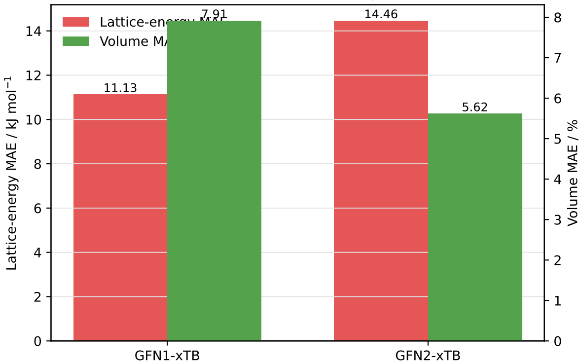
X23b native Bloch k222 cell optimization
