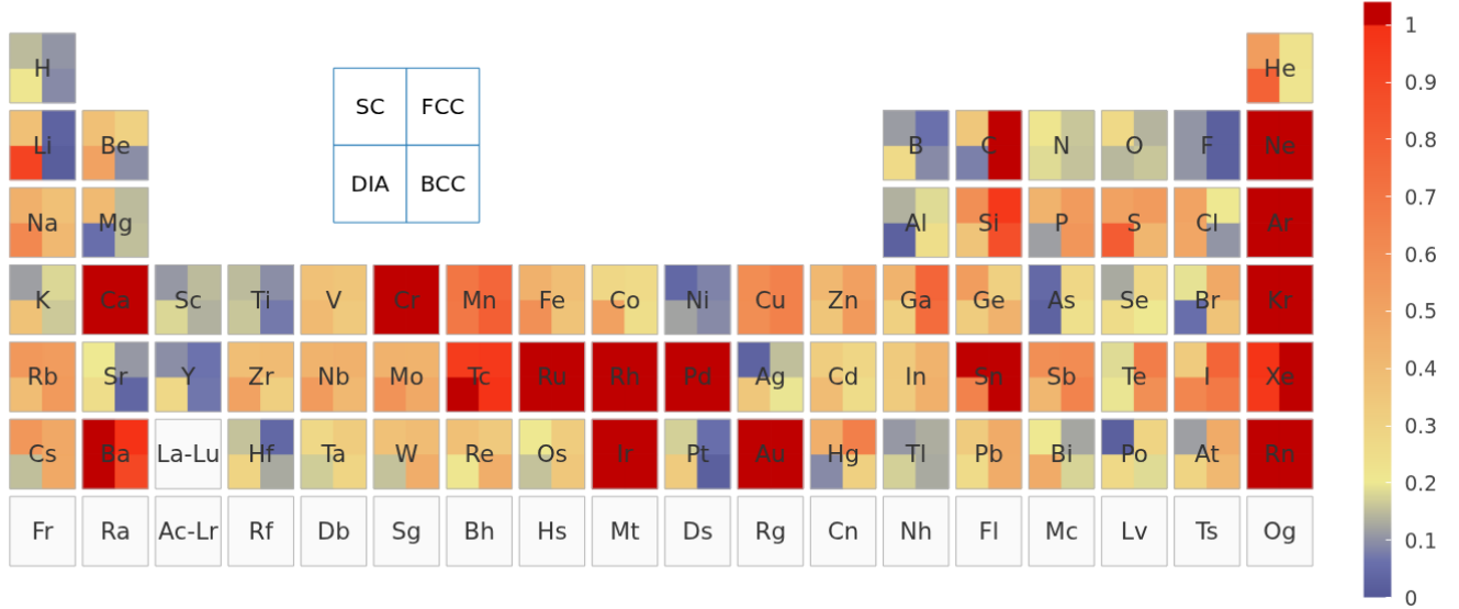
FIG. 4. Total equation-of-state error of the original CP2K-GTH-UZH settings relative to SIRIUS-FP-LAPW, expressed with the \epsilon metric of Eq. (11). This comparison contains both Gaussian-basis and pseudopotential errors.
