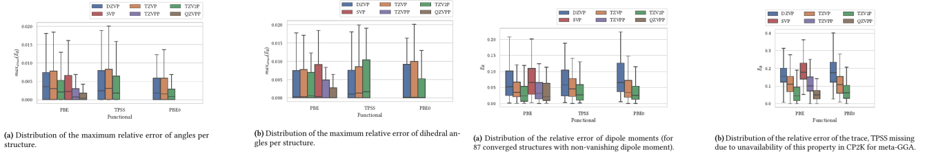
FIG. 3. Molecular calibration beyond bond lengths. Left: relative errors for nonlinear and dihedral angles. Right: relative errors for dipole moments and average molecular polarizabilities. Response properties are more demanding than equilibrium bond lengths, but they retain the systematic basis-set improvement needed before transferring the basis to periodic verification.
