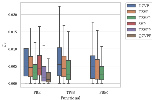
FIG. 2. Relative bond-length errors for the molecular calibration set. The error is E_R = |d_{\text{CP2K}} - d_{\text{G16}}|/|d_{\text{G16}}| , where d_{\text{G16}} is the Gaussian 16/def2-QZVP all-electron reference bond length. DZVP, TZVP, and TZV2P are CP2K/GPW calculations with GTH-UZH pseudopotentials. In the PBE panel, SVP, TZVPP, and QZVPP are CP2K/GAPW all-electron calculations with corresponding UZH-MOLOPT basis sets and provide an internal all-electron CP2K comparison. Outliers are omitted to emphasize median and interquartile behavior.
