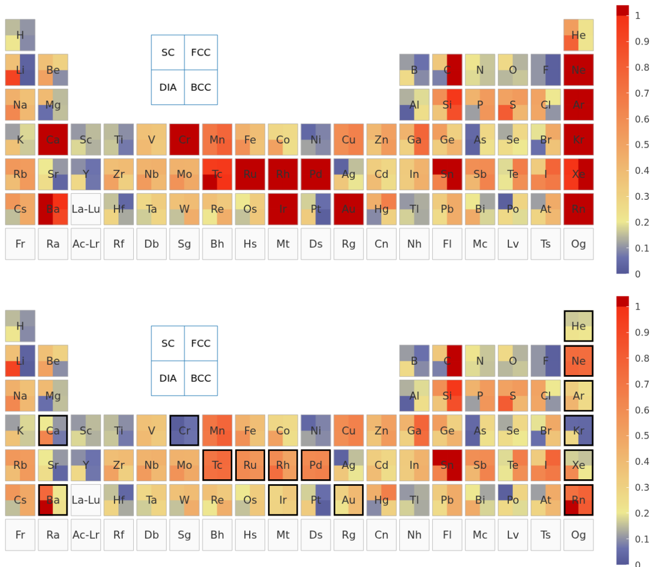
FIG. 4. Total equation-of-state error relative to SIRIUS-FP-LAPW, expressed with the \varepsilon metric of Eq. (12). Top: original CP2K-GTH-UZH settings. Bottom: completed view in which entries absent from the improved data set are filled with the corresponding original CP2K-GTH-UZH values; black frames mark the recomputed improved entries. Each map contains both Gaussian-basis and pseudopotential errors and therefore represents the practical production-level CP2K error before and after applying the UZH protocol.
