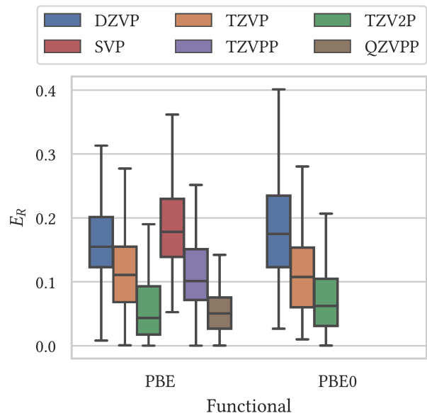
FIG. 3. Relative errors for average molecular polarizabilities, E_R = |\bar{\alpha}_{\text{CP2K}} - \bar{\alpha}_{\text{G16}}|/|\bar{\alpha}_{\text{G16}}| . Polarizabilities are the most demanding molecular response test in this set because they require sufficient diffuse flexibility; meta-generalized-gradient data are omitted because this property was not available for the corresponding CP2K calculations.
