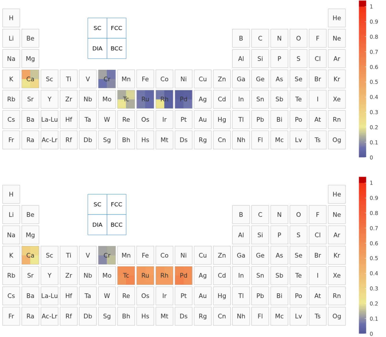
FIG. 6. Residual error decomposition for the optimized UZH settings. Top: CP2K-GTH-UZH-new relative to SIRIUS-GTH-UZH-new, which isolates the remaining Gaussian-basis contribution. Bottom: SIRIUS-GTH-UZH-new relative to SIRIUS-FP-LAPW, which isolates the remaining pseudopotential contribution.
