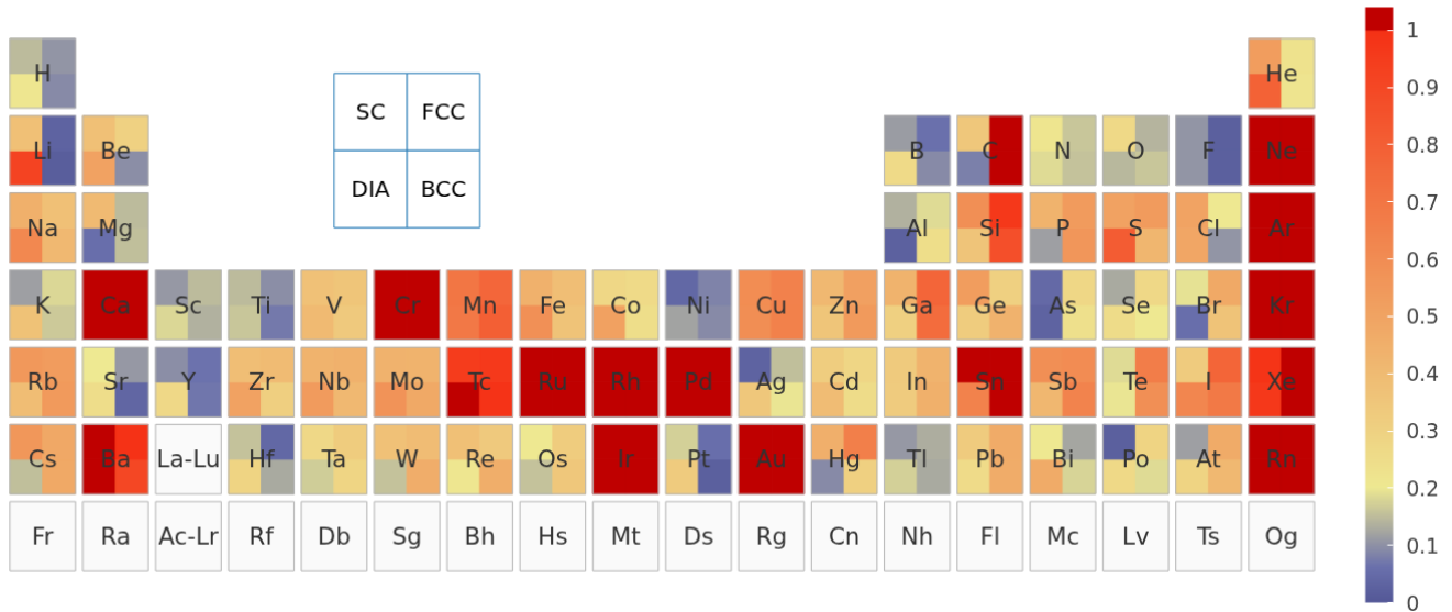
FIG. 4. Total equation-of-state error of the original CP2K-GTH-UZH settings relative to SIRIUS-FP-LAPW, expressed with the \epsilon metric of Eq. (10). This comparison contains both Gaussian-basis and pseudopotential errors.
