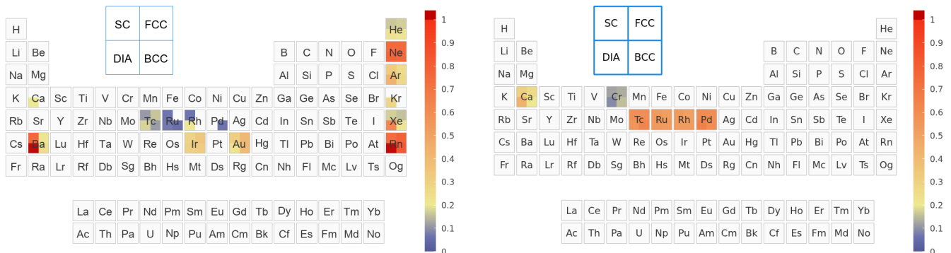
FIG. 6. Left: illustrative estimate of the residual CP2K Gaussian-basis contribution after improvement, constructed as \max[\epsilon_{\text{total}} - \epsilon_{\text{pp}}, 0] from Fig. 7 and the residual pseudopotential map. Right: residual pseudopotential error for the improved UZH settings, obtained from SIRIUS-GTH-UZH-new relative to the SIRIUS-FP-LAPW reference.
