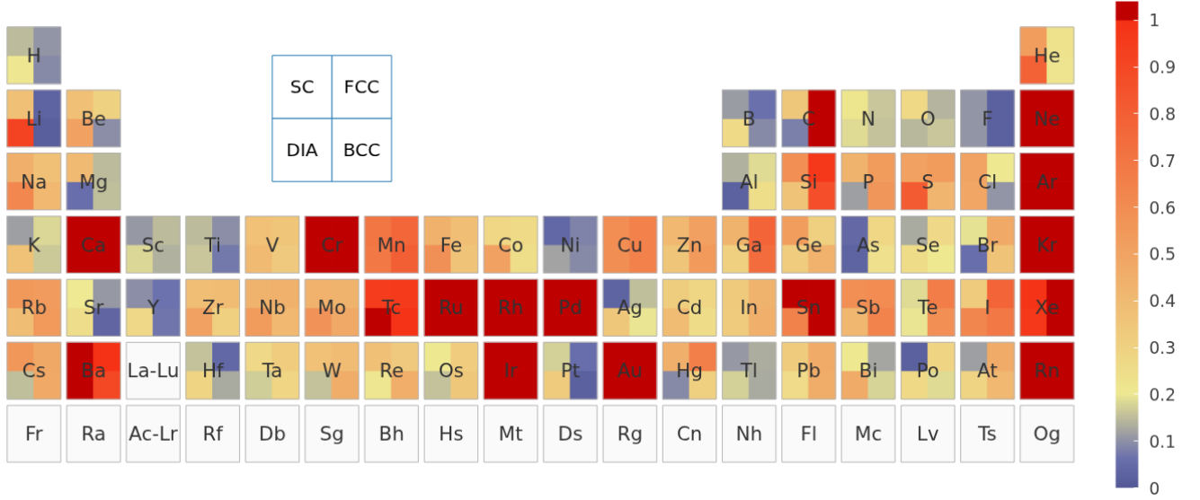
FIG. 4. Total equation-of-state error of the original CP2K-GTH-UZH settings relative to SIRIUS-FP-LAPW, expressed with the \varepsilon metric of Eq. (10). This comparison contains both Gaussian-basis and pseudopotential errors.
