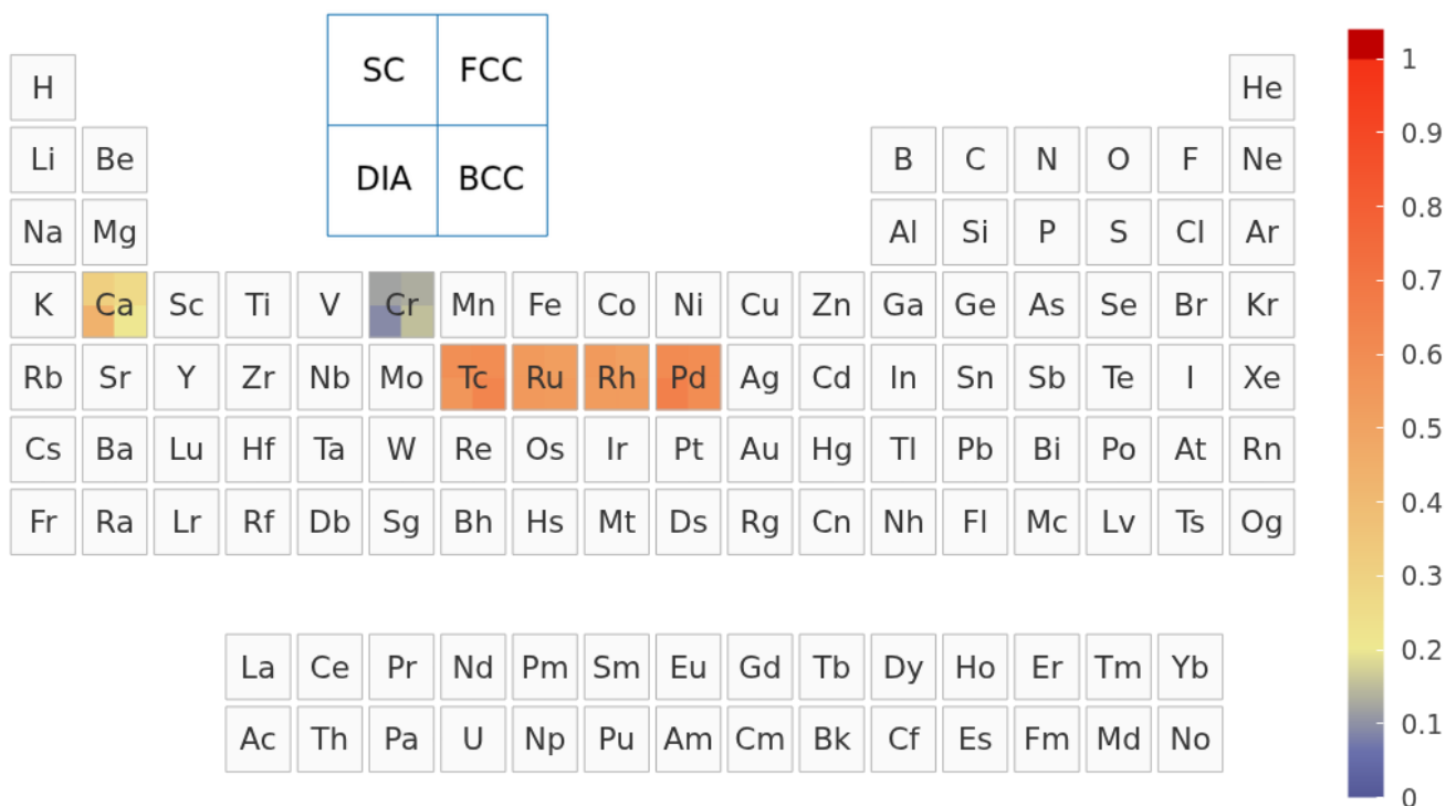
FIG. 6. Optimized UZH error decomposition. Top: CP2K-GTH-UZH-new relative to SIRIUS-GTH-UZH-new, i.e., the Gaussian-basis component after optimization. Bottom: SIRIUS-GTH-UZH-new relative to SIRIUS-FP-LAPW, i.e., the pseudopotential component after optimization.
