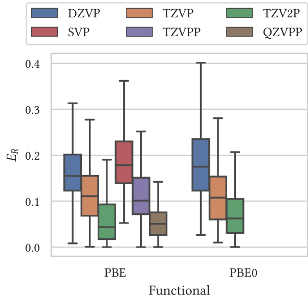
FIG. 3. Distribution of relative errors for average molecular polarizabilities, adapted from Fig. 4.11 of Ref. [22]. Polarizabilities are the most demanding molecular response test in this set because they require sufficient diffuse flexibility; TPSS is omitted because this property was not available for meta-generalized-gradient calculations in CP2K.
