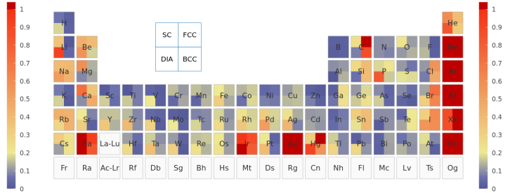
FIG. 5. Error decomposition for the original UZH settings. Left: SIRIUS-GTH-UZH relative to SIRIUS-FP-LAPW, which isolates the pseudopotential error. Right: CP2K-GTH-UZH relative to SIRIUS-GTH-UZH, which isolates the Gaussian-basis error.
