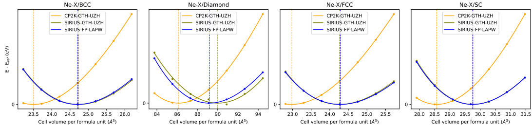
FIG. 11. Representative equation-of-state curves for Ne. Noble gases are sensitive tests of diffuse basis flexibility because their equation-of-state curves are shallow.
