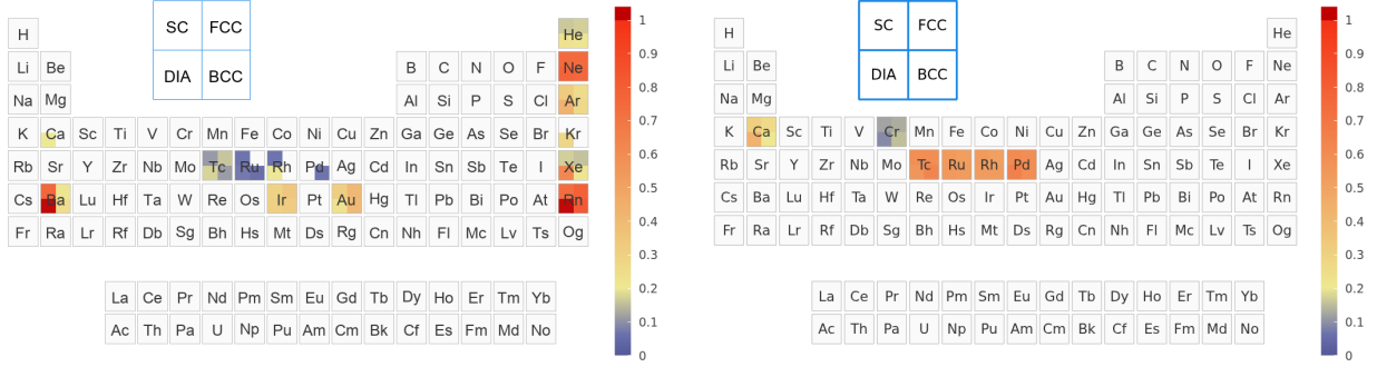
FIG. 7. Residual diagnostic for the improved settings. Left: illustrative estimate of the residual CP2K Gaussian-basis contribution, constructed as the positive difference between the final CP2K-GTH-UZH-new total-error map and the residual pseudopotential map. Right: residual pseudopotential error for the improved SIRIUS-GTH-UZH-new settings relative to the SIRIUS-FP-LAPW reference. The left panel is a diagnostic estimate rather than a direct CP2K-GTH-UZH-new/SIRIUS-GTH-UZH-new equation-of-state comparison.
