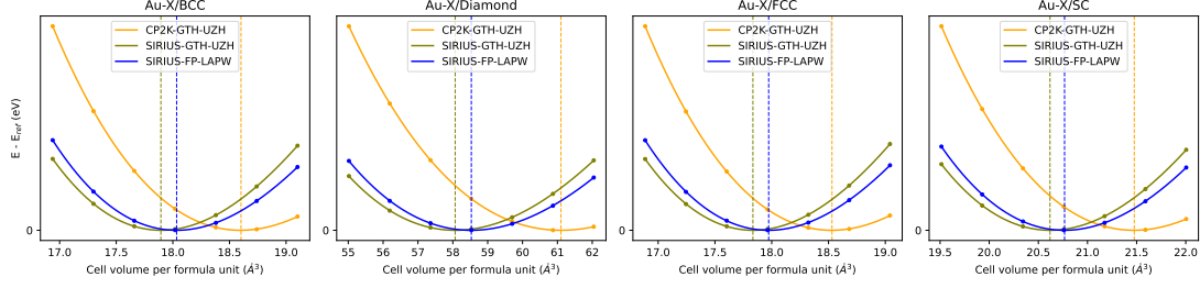
FIG. 12. Representative equation-of-state curves for Au, illustrating the behavior of a heavy element where basis completeness and relativistic pseudopotential transferability must both be monitored.
