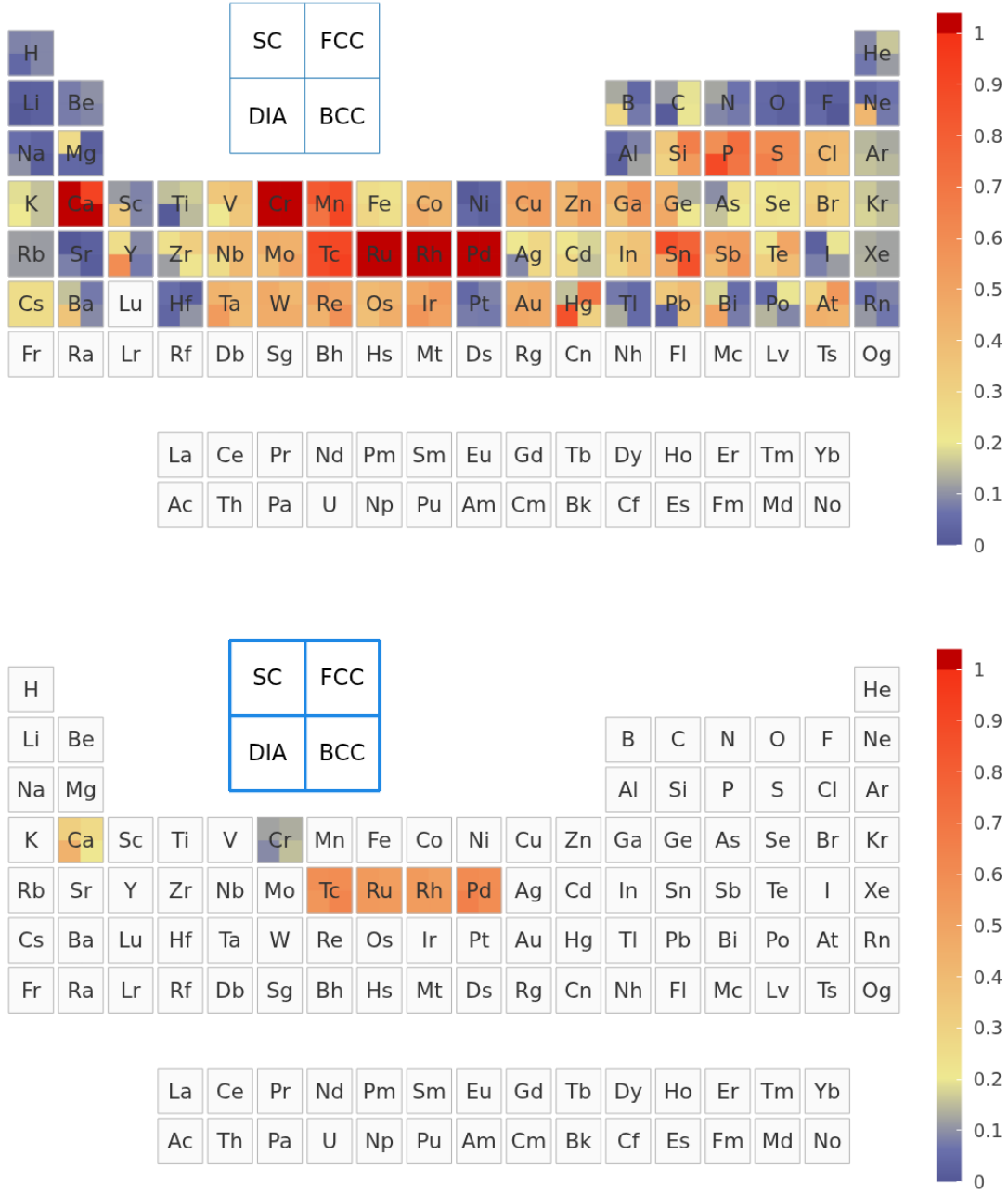
FIG. 6. Pseudopotential contribution before and after applying the UZH protocol. Top: original SIRSUS-GTH-UZH settings relative to SIRSUS-FP-LAPW. Bottom: improved SIRSUS-GTH-UZH-new settings relative to SIRSUS-FP-LAPW. Because both panels use SIRSUS on the pseudopotential side, the CP2K Gaussian basis is absent and the comparison isolates the pseudopotential transferability error.
