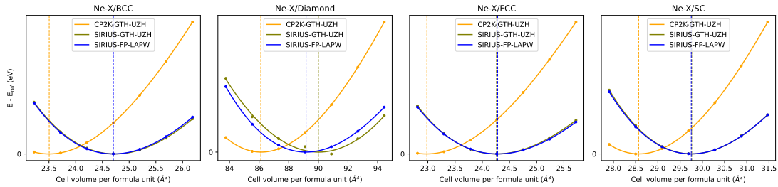
FIG. 7. Representative equation-of-state curves for Ne. Noble gases are sensitive tests of diffuse basis flexibility because their equation-of-state curves are shallow.
