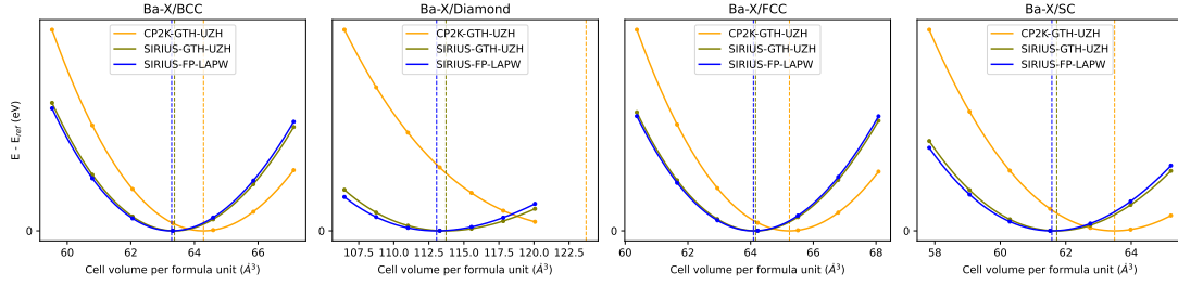
FIG. 6. Representative equation-of-state curves for Ba. The comparison highlights a case with a substantial Gaussian-basis contribution in the original CP2K-GTH-UZH settings.
