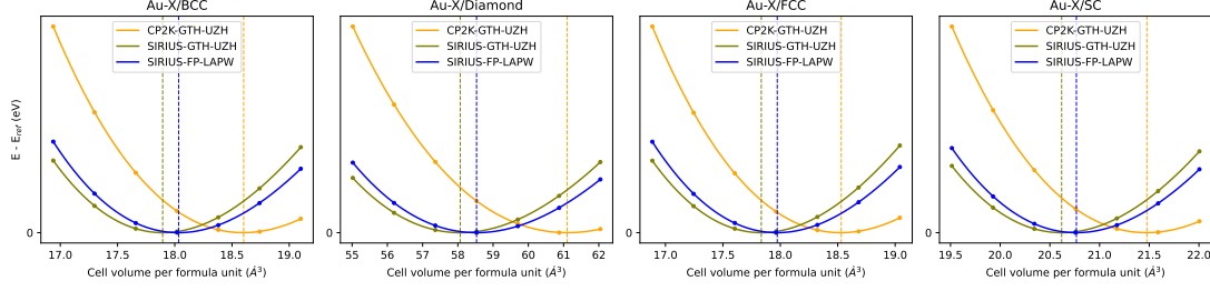
FIG. 8. Representative equation-of-state curves for Au, illustrating the behavior of a heavy element where basis completeness and relativistic pseudopotential transferability must both be monitored.
