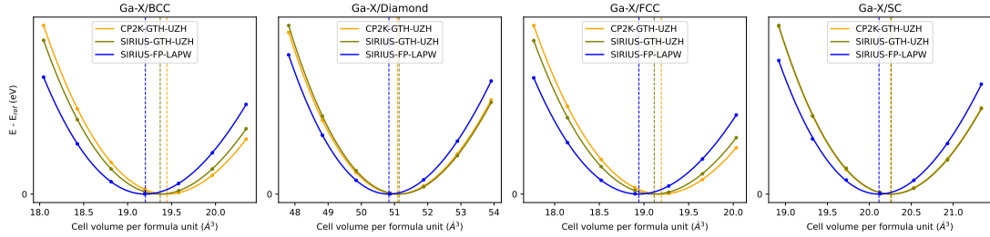
FIG. 9. Representative equation-of-state curves for Ga.
