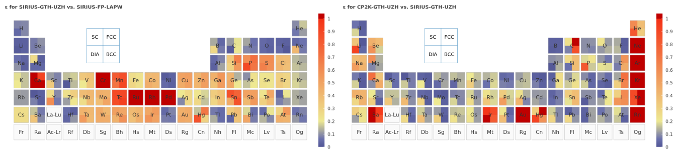
FIG. 6. Error decomposition for the original UZH settings. Right: CP2K-GTH-UZH relative to SIRIUS-GTH-UZH, which isolates the Gaussian-basis error. Left: SIRIUS-GTH-UZH relative to SIRIUS-FP-LAPW, which isolates the pseudopotential error.
