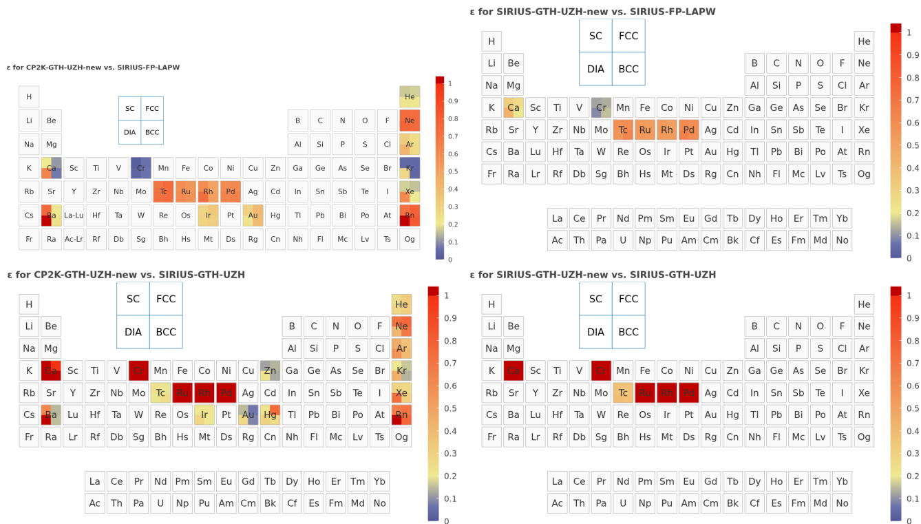
FIG. 7. Verification of the improved UZH settings. Top left: total CP2K-GTH-UZH-new error relative to SIRIUS-FP-LAPW. Bottom left: residual CP2K Gaussian-basis error. Top right: residual pseudopotential error after improvement. Bottom left: residual CP2K Gaussian-basis error. Bottom right: direct comparison of new and original SIRIUS-GTH-UZH pseudopotential settings.
