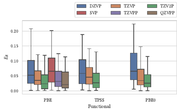
FIG. 3. Molecular calibration of response properties. The distributions show relative errors for dipole moments and average molecular polarizabilities. Response properties are more demanding than equilibrium bond lengths, but they retain the systematic basis-set improvement needed before transferring the basis to periodic verification. Distribution of relative errors for molecular dipole moments. The statistics include converged structures with non-vanishing dipole moments and show that response-sensitive density properties retain the same systematic basis-set improvement observed for structural observables.
