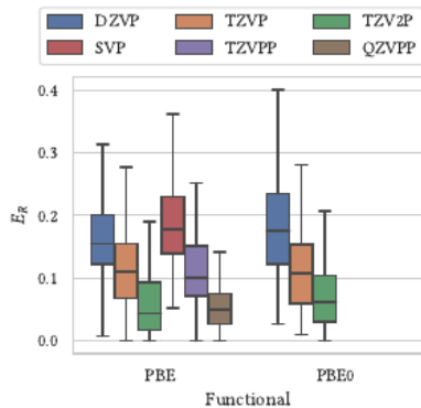
FIG. 4. Distribution of relative errors for average molecular polarizabilities. Polarizabilities are the most demanding molecular response test in this set because they require sufficient diffuse flexibility; TPSS is omitted because this property was not available for meta-generalized-gradient calculations in CP2K.
