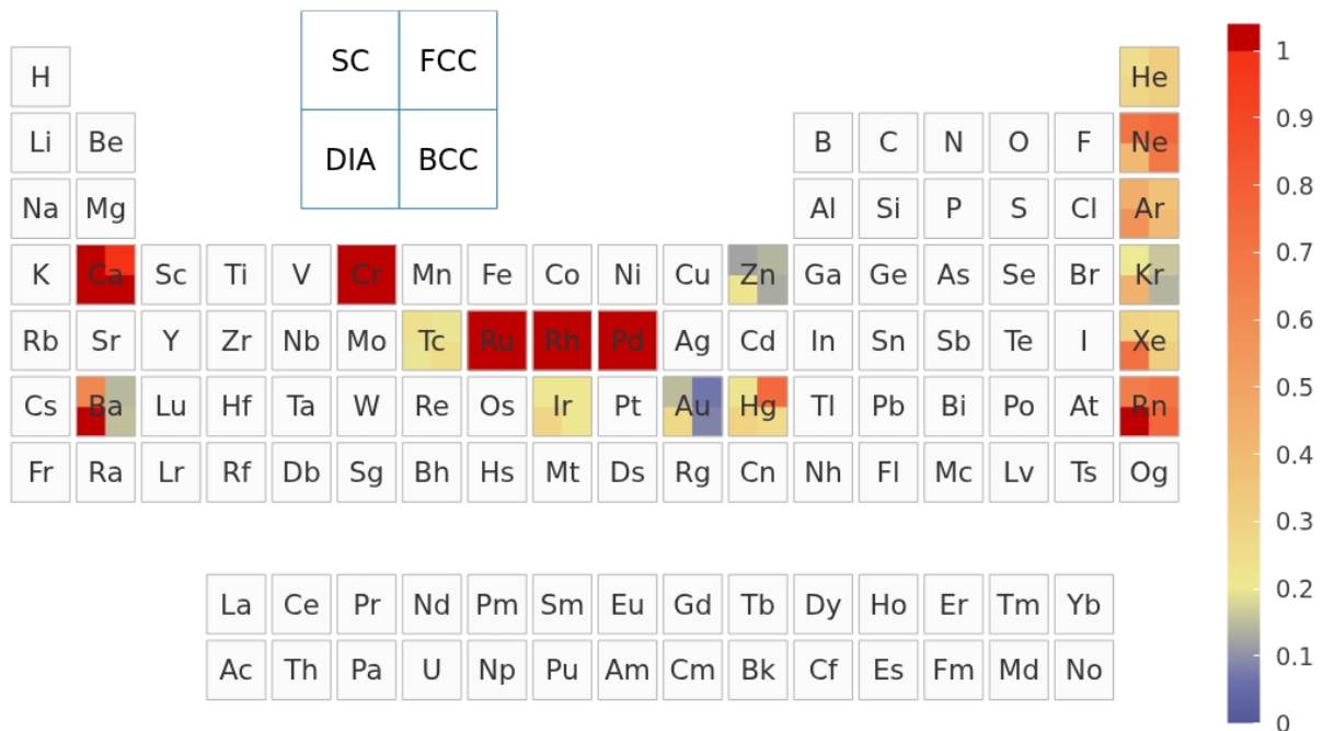
FIG. 7. Mixed diagnostic comparing CP2K-GTH-UZH-new with the original SIRIUS-GTH-UZH reference. This comparison is not a residual basis-set error because it combines the remaining CP2K Gaussian-basis contribution with the change from the original to the improved pseudopotential settings.
