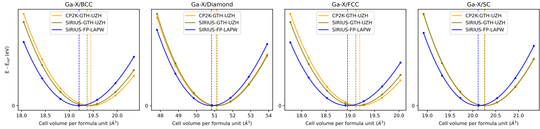
FIG. 12. Representative equation-of-state curves for Ga.
