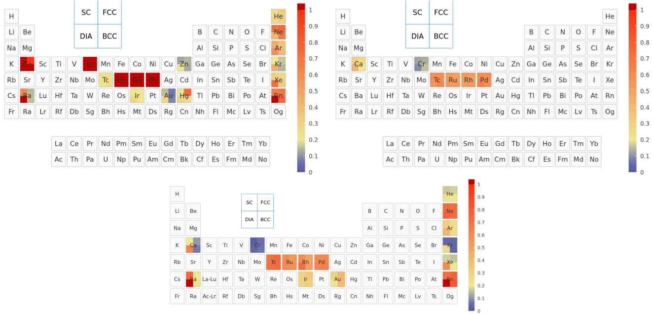
FIG. 6. Verification of the improved UZH settings. Top left: residual CP2K Gaussian-basis error, obtained from CP2K-GTH-UZH-new relative to SIRIUS-GTH-UZH. Top right: residual pseudopotential error, obtained from SIRIUS-GTH-UZH-new relative to SIRIUS-FP-LAPW. Bottom: total CP2K-GTH-UZH-new error relative to SIRIUS-FP-LAPW.
