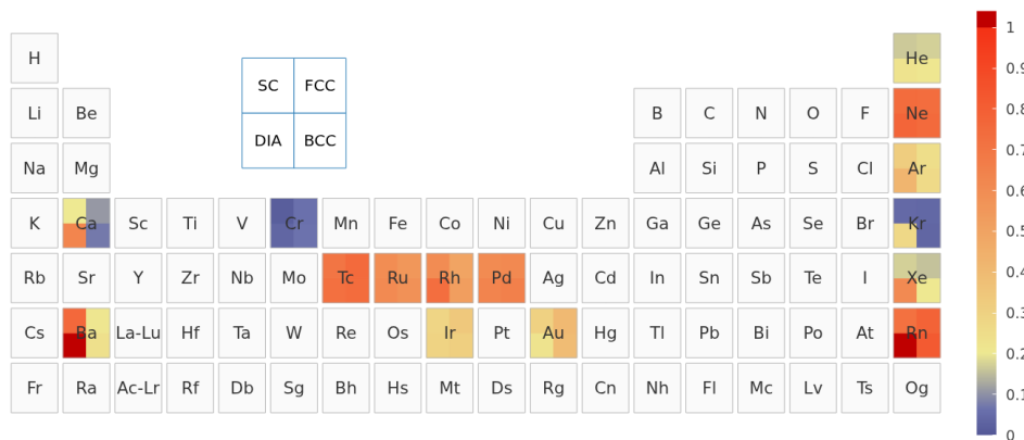
FIG. 7. Total equation-of-state error of the improved CP2K-GTH-UZH-new settings relative to SIRIUS-FP-LAPW. This comparison is the final production-level accuracy test and contains the remaining CP2K Gaussian-basis contribution together with the residual pseudopotential error shown in Fig. 6.
