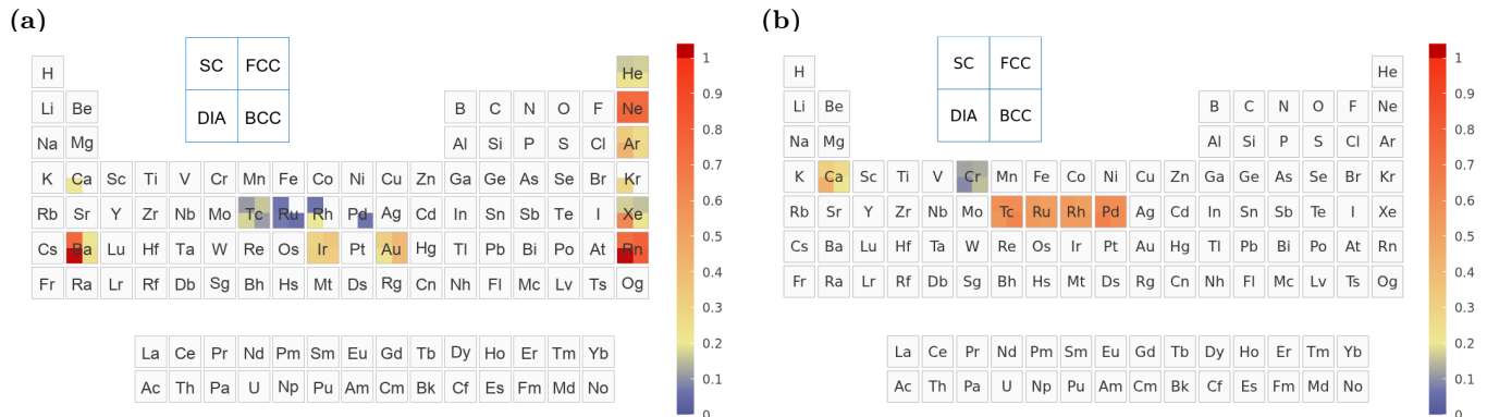
FIG. 6. (a) Illustrative estimate of the residual CP2K Gaussian-basis contribution after improvement, constructed as \max[\epsilon_{\text{total}} - \epsilon_{\text{pp}}, 0] from Fig. 7 and panel (b). (b) Residual pseudopotential error for the improved UZH settings, obtained from SIRIUS-GTH-UZH-new relative to the SIRIUS-FP-LAPW reference.
