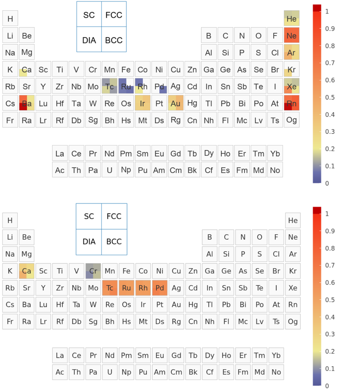
FIG. 6. Residual component diagnostics for the improved UZH settings. Top: residual CP2K Gaussian-basis contribution, constructed as the positive difference between the final CP2K-GTH-UZH-new total-error map and the residual pseudopotential map. Bottom: residual pseudopotential error for the improved SIRIUS-GTH-UZH-new settings relative to the SIRIUS-FP-LAPW reference.
