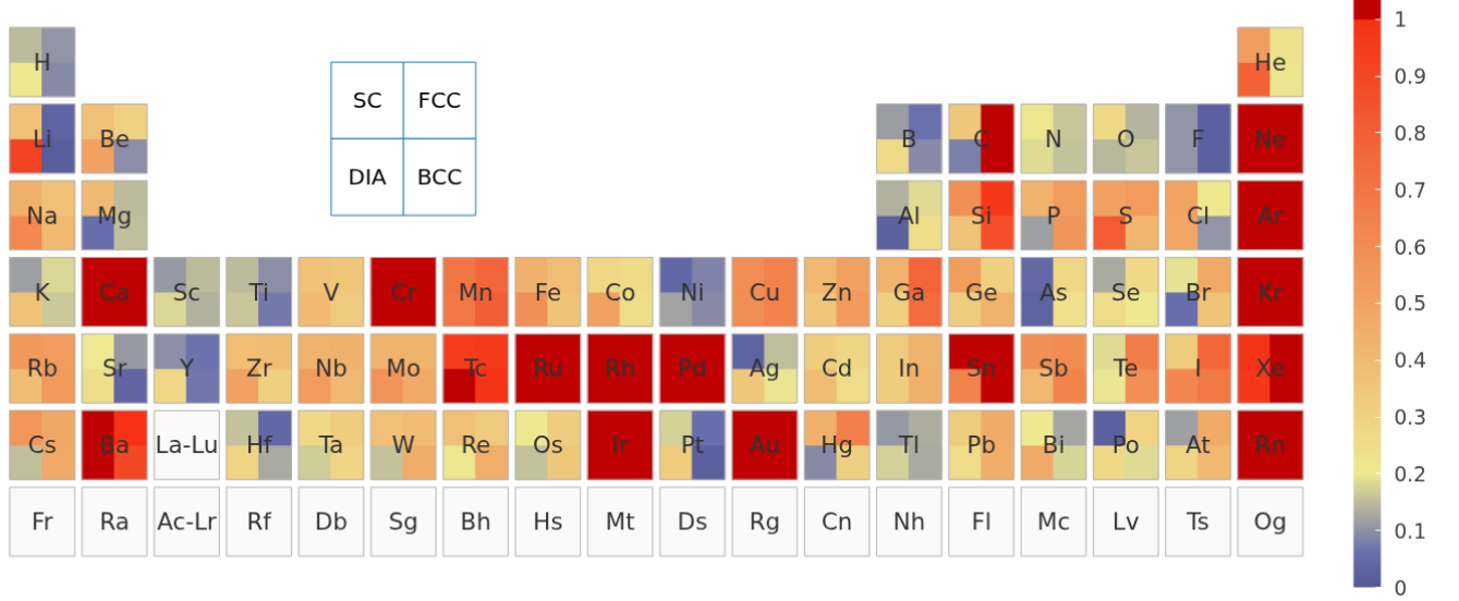
FIG. 4. Total equation-of-state error of the original CP2K-GTH-UZH settings relative to SIRIUS-FP-LAPW, expressed with the \epsilon metric of Eq. (11). This comparison contains both Gaussian-basis and pseudopotential errors.
