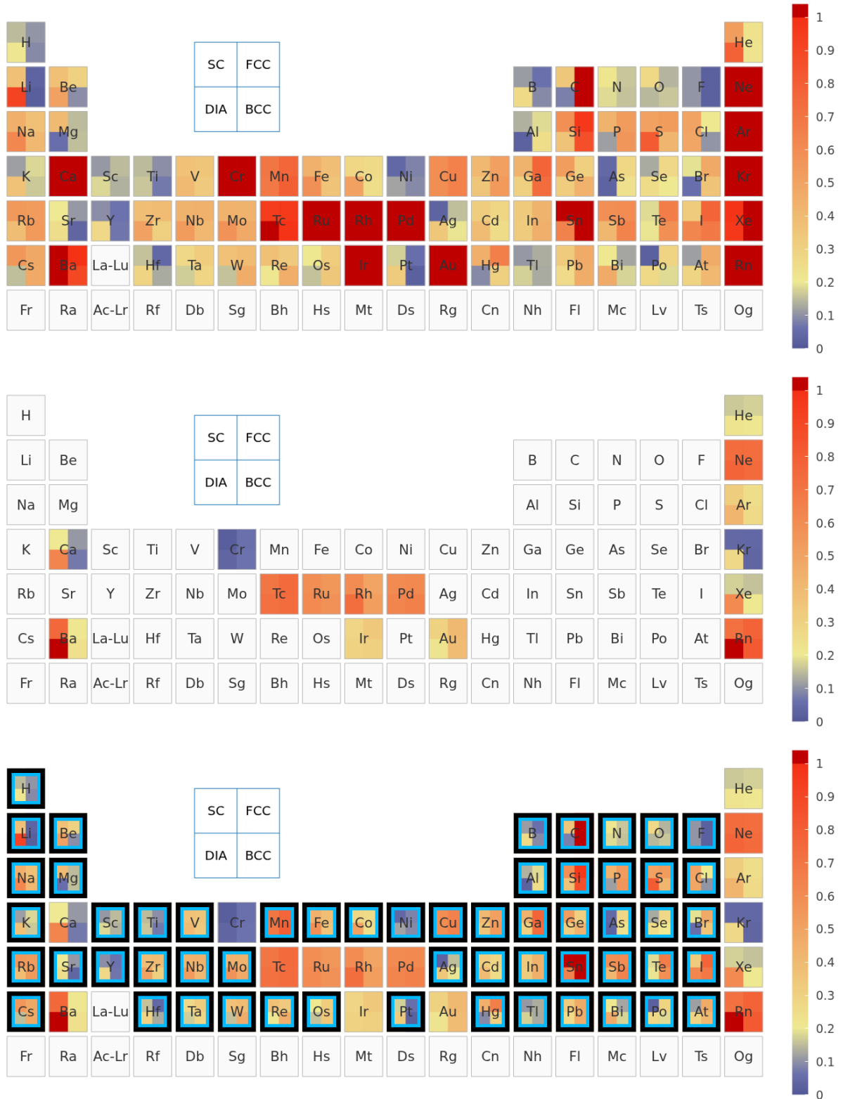
FIG. 4. Total equation-of-state error relative to SIRIUS-FP-LAPW, expressed with the \varepsilon metric of Eq. (10). Top: original CP2K-GTH-UZH settings. Middle: improved CP2K-GTH-UZH-new settings. Bottom: completed view in which entries absent from the improved data set are filled with the corresponding original CP2K-GTH-UZH values; black-cyan frames mark the retained original entries. Each map contains both Gaussian-basis and pseudopotential errors and therefore represents the practical production-level CP2K error before and after applying the UZH protocol.
