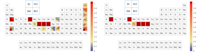
FIG. 6. Residual component errors after applying the UZH protocol. Left: illustrative estimate of the residual CP2K Gaussian-basis contribution, constructed as the positive difference between the final CP2K-GTH-UZH-new total-error map and the residual pseudopotential map. Right: residual pseudopotential error for the improved SIRIUS-GTH-UZH-new settings relative to the SIRIUS-FP-LAPW reference. Component-update diagnostics for the improved UZH settings. Left: CP2K-side basis-set-update diagnostic, obtained from CP2K-GTH-UZH-new relative to the original SIRIUS-GTH-UZH reference. Right: direct pseudopotential-update diagnostic, obtained from SIRIUS-GTH-UZH-new relative to the original SIRIUS-GTH-UZH settings.
