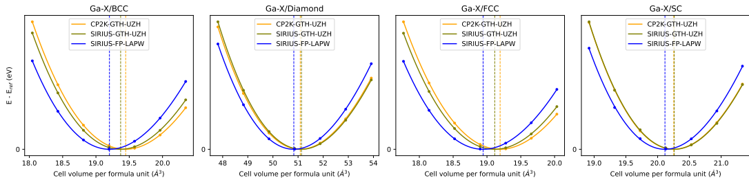
FIG. 6. Representative equation-of-state curves for Ga.
