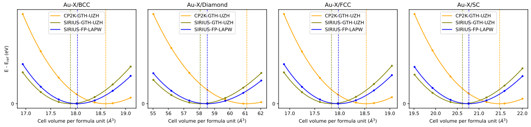
FIG. 5. Representative equation-of-state curves for Au, illustrating the behavior of a heavy element where basis completeness and relativistic pseudopotential transferability must both be monitored.
