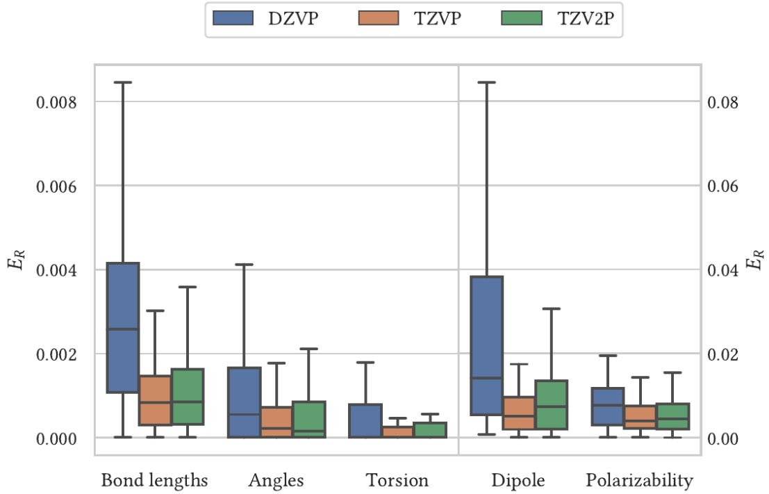
FIG. 1. Additional molecular benchmark statistics for properties that are more sensitive to basis flexibility. Direct comparison of PBE0 calculations performed without and with the auxiliary density matrix method for the same UZH-MOLOPT basis levels. Geometric observables remain close, while dipoles and polarizabilities provide the more sensitive tests of the auxiliary basis.
