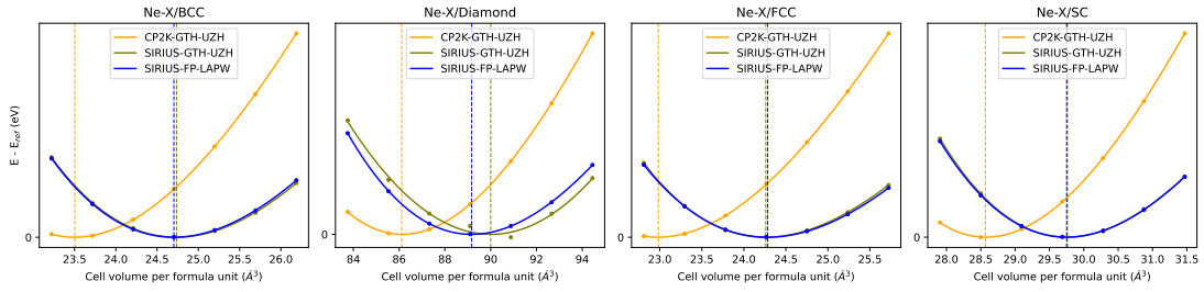
FIG. 4. Representative equation-of-state curves for Ne. Noble gases are sensitive tests of diffuse basis flexibility because their equation-of-state curves are shallow.
