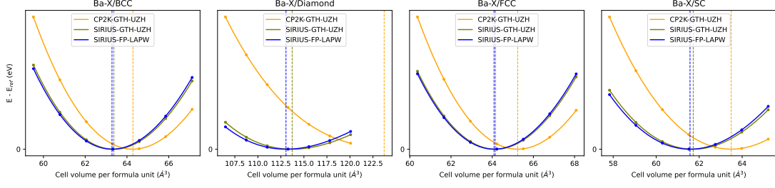
FIG. 3. Representative equation-of-state curves for Ba. The comparison highlights a case with a substantial Gaussian-basis contribution in the original CP2K-GTH-UZH settings.
