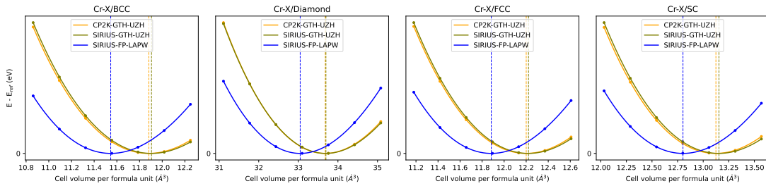
FIG. 2. Representative equation-of-state curves for Cr. The behavior is characteristic of a pseudopotential-limited case in the original settings.
