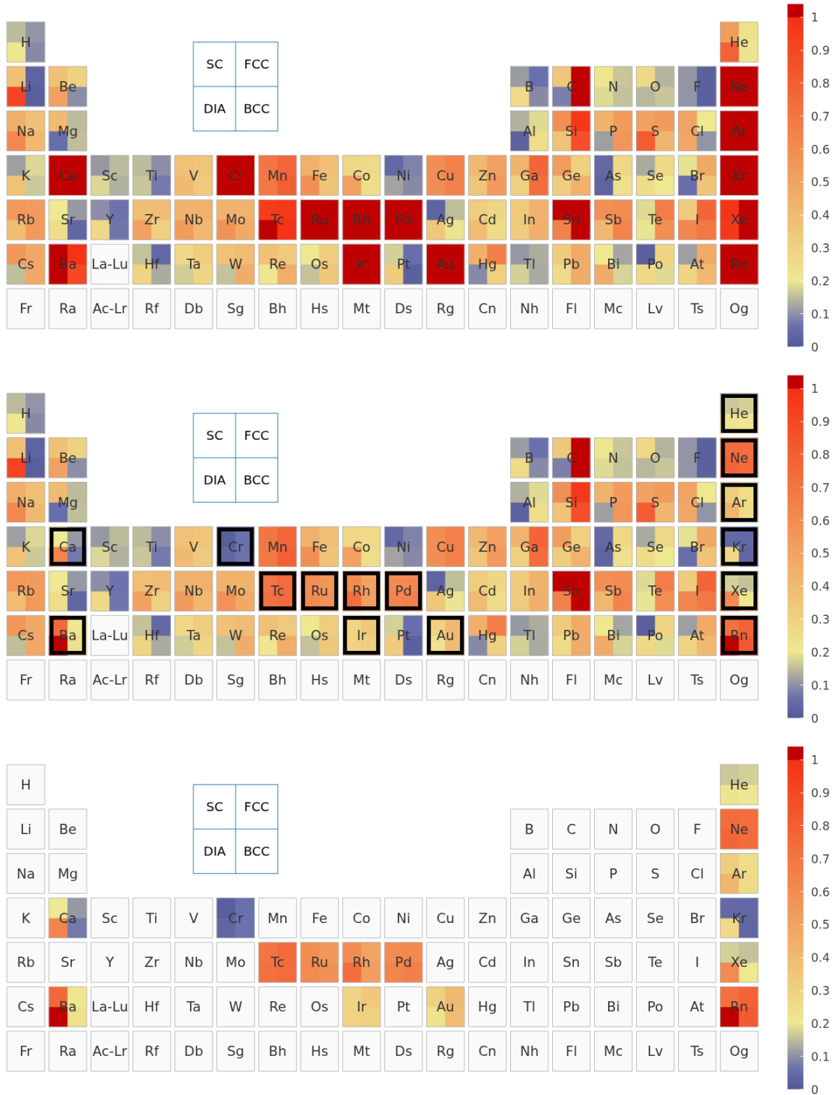
FIG. 4. Total equation-of-state error relative to SIRIUS-FP-LAPW, expressed with the \varepsilon metric of Eq. (10). Top: original CP2K-GTH-UZH settings. Middle: completed view in which entries absent from the improved data set are filled with the corresponding original CP2K-GTH-UZH values; black frames mark the recomputed improved entries. Bottom: improved CP2K-GTH-UZH-new settings. Each map contains both Gaussian-basis and pseudopotential errors and therefore represents the practical production-level CP2K error before and after applying the UZH protocol.
