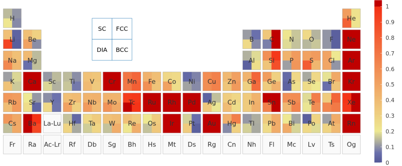
FIG. 4. Total equation-of-state error of the original CP2K-GTH-UZH settings relative to SIRIUS-FP-LAPW, expressed with the \epsilon metric of Eq. (12). This comparison contains both Gaussian-basis and pseudopotential errors.
