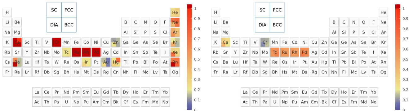
FIG. 6. Residual error decomposition for the improved UZH settings. Left: residual CP2K Gaussian-basis error, obtained from CP2K-GTH-UZH-new relative to SIRIUS-GTH-UZH. Right: residual pseudopotential error, obtained from SIRIUS-GTH-UZH-new relative to SIRIUS-FP-LAPW.
