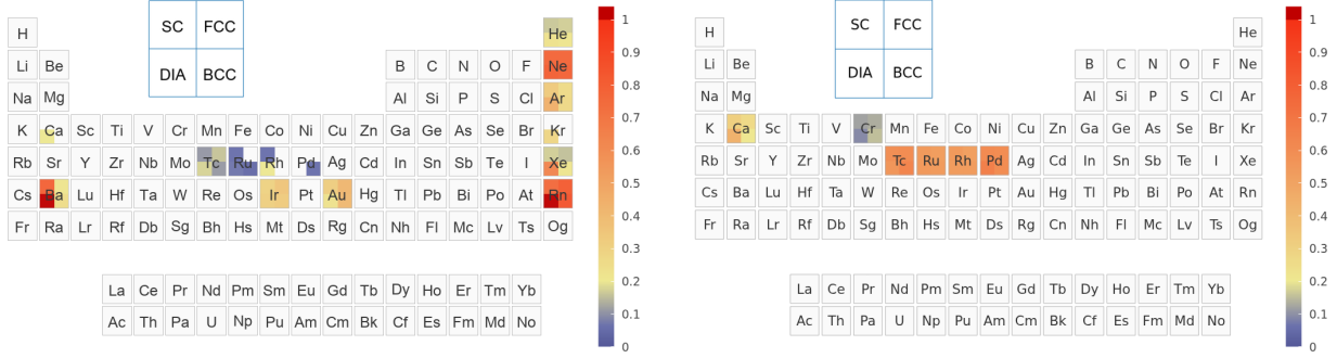
FIG. 6. Residual diagnostic for the improved settings. Left: illustrative estimate of the residual CP2K Gaussian-basis contribution, constructed as the positive difference between the final CP2K-GTH-UZH-new total-error map and the residual pseudopotential map. Right: residual pseudopotential error for the improved SIRIUS-GTH-UZH-new settings relative to the SIRIUS-FP-LAPW reference. The left panel is a diagnostic estimate rather than a direct CP2K-GTH-UZH-new/SIRIUS-GTH-UZH-new equation-of-state comparison.
