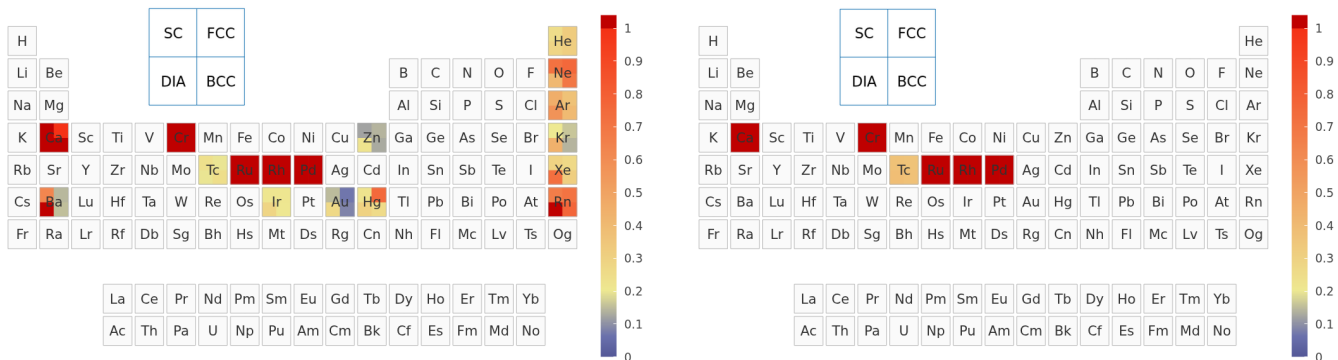
FIG. 6. Component-update diagnostics for the improved UZH settings. Left: CP2K-side basis-set-update diagnostic, obtained from CP2K-GTH-UZH-new relative to the original SIRIUS-GTH-UZH reference. Right: direct pseudopotential-update diagnostic, obtained from SIRIUS-GTH-UZH-new relative to the original SIRIUS-GTH-UZH settings.
