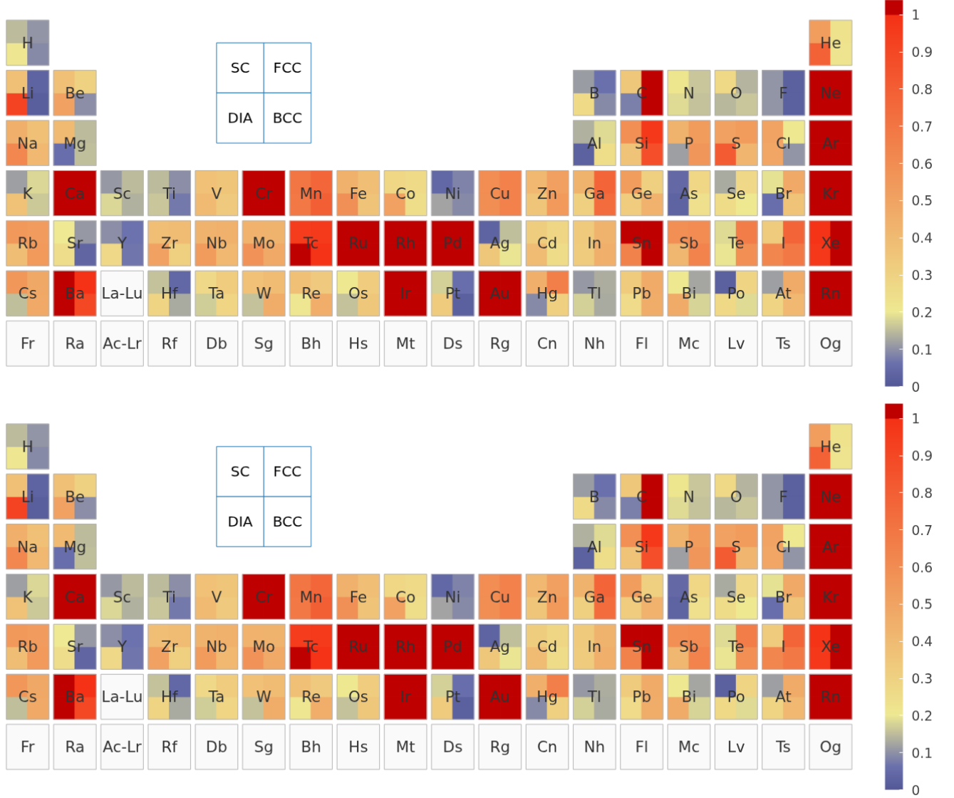
\epsilon for CP2K-GTH-UZH vs. SIRIUS-FP-LAPW
