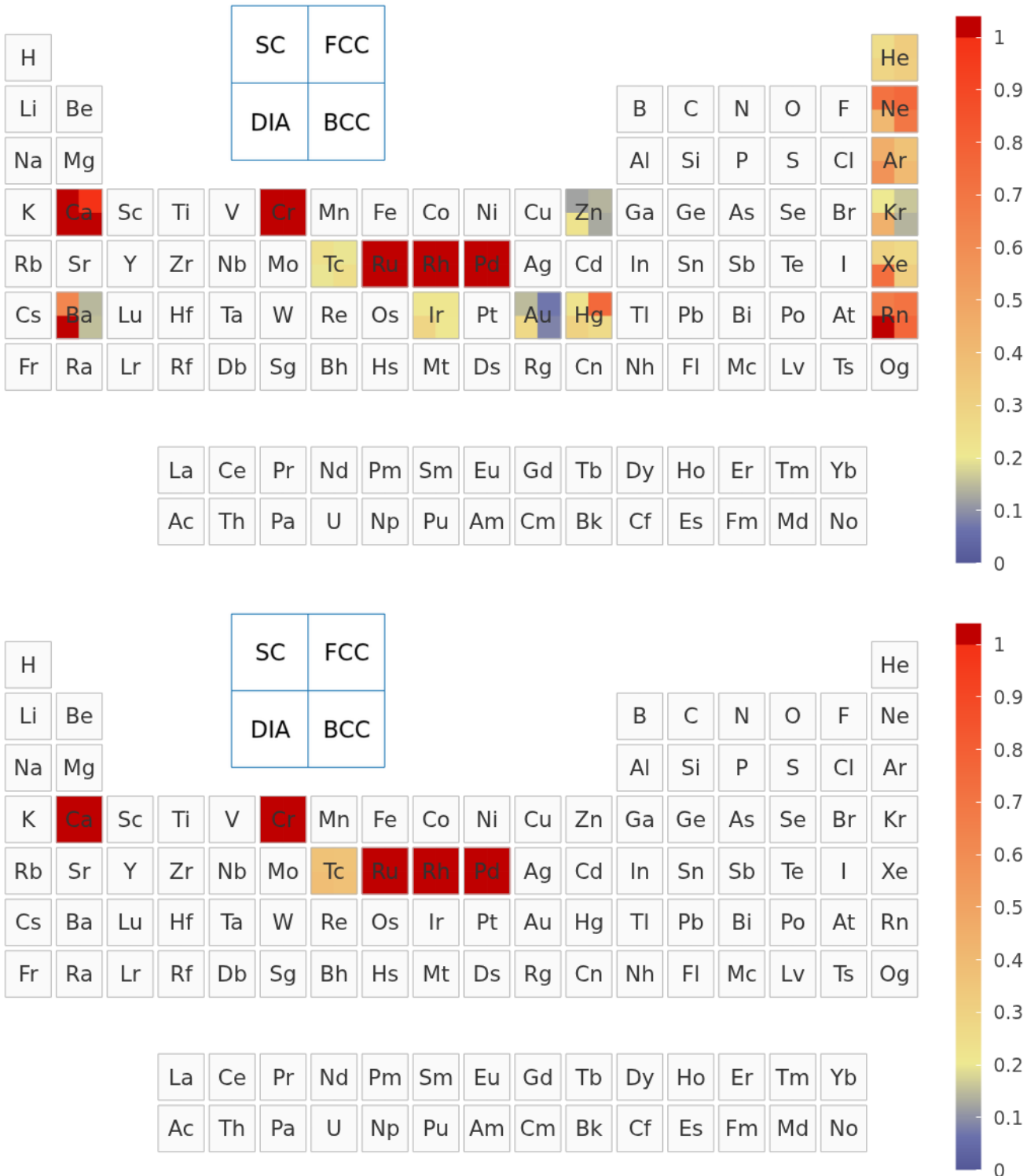
FIG. 6. Component-update diagnostics for the improved UZH settings. Top: CP2K-side basis-set-update diagnostic, obtained from CP2K-GTH-UZH-new relative to the original SIRIUS-GTH-UZH reference. Bottom: direct pseudopotential-update diagnostic, obtained from SIRIUS-GTH-UZH-new relative to the original SIRIUS-GTH-UZH settings.
