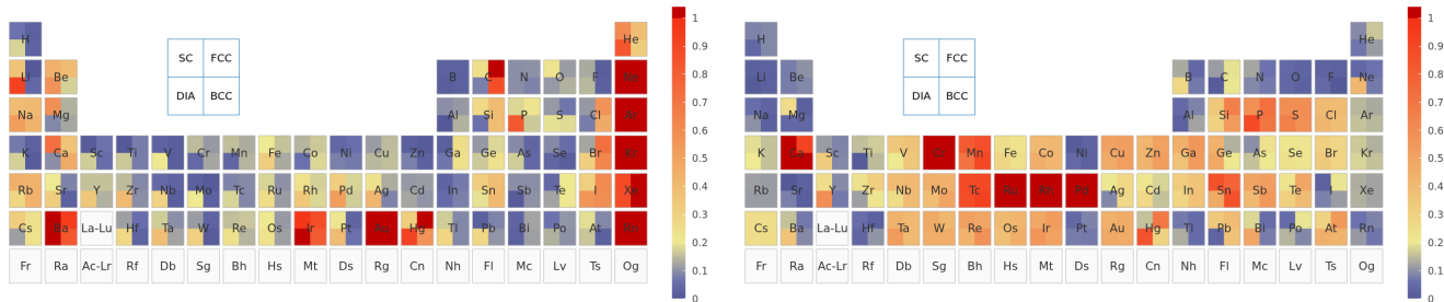
FIG. 5. Error decomposition for the original UZH settings. Left: CP2K-GTH-UZH relative to SIRIUS-GTH-UZH, which isolates the Gaussian-basis error. Right: SIRIUS-GTH-UZH relative to SIRIUS-FP-LAPW, which isolates the pseudopotential error.
