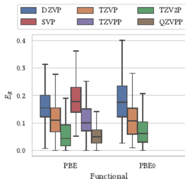
FIG. 6. Distribution of relative errors for average molecular polarizabilities. Polarizabilities are the most demanding molecular response test in this set because they require sufficient diffuse flexibility; TPSS is omitted because this property was not available for meta-generalized-gradient calculations in CP2K.
