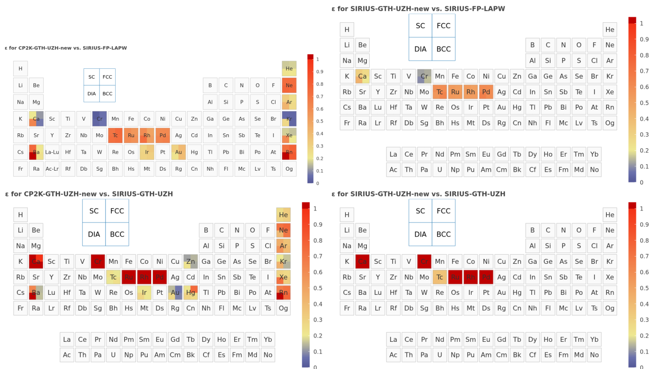
FIG. 9. Verification of the improved UZH settings. Top left: total CP2K-GTH-UZH-new error relative to SIRIUS-FP-LAPW. Bottom left: residual CP2K Gaussian-basis error. Top right: residual pseudopotential error after improvement. Bottom right: direct comparison of new and original SIRIUS-GTH-UZH pseudopotential settings.
