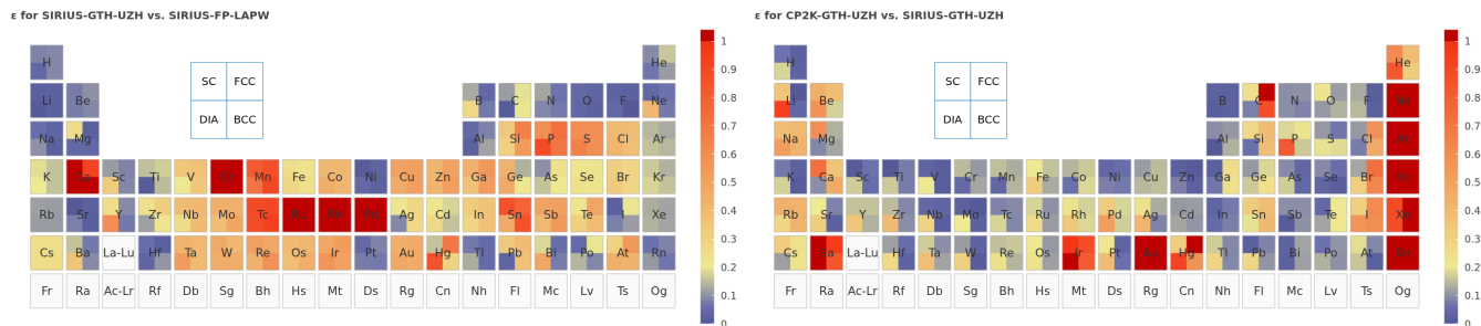
FIG. 8. Error decomposition for the original UZH settings. Right: CP2K-GTH-UZH relative to SIRIUS-GTH-UZH, which isolates the Gaussian-basis error. Left: SIRIUS-GTH-UZH relative to SIRIUS-FP-LAPW, which isolates the pseudopotential error.
