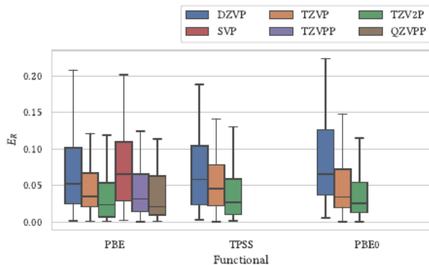
FIG. 5. Distribution of relative errors for molecular dipole moments. The statistics include converged structures with non-vanishing dipole moments and show that response-sensitive density properties retain the same systematic basis-set improvement observed for structural observables.
