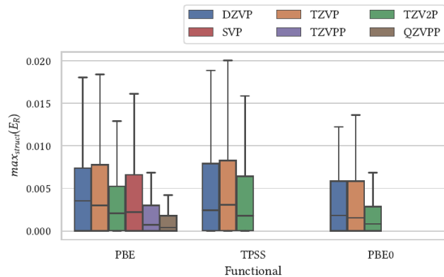
FIG. 3. Distribution of relative errors for nonlinear angles in the molecular calibration set. Angular observables are more sensitive than bond lengths to automated atom matching and near-symmetric geometries, but the systematic improvement from DZVP to TZV2P remains visible.
