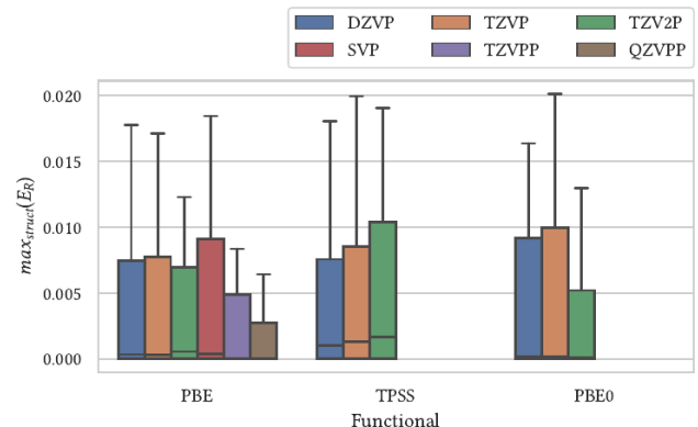
FIG. 4. Distribution of relative errors for dihedral angles in the molecular calibration set. The broader tails reflect the stronger sensitivity of torsional coordinates to small structural and matching differences, while the basis-set hierarchy remains consistent with the bond-length and angle tests.
