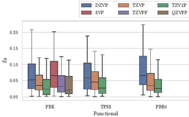
FIG. 5. Molecular calibration of response properties. The distributions show relative errors for dipole moments and average molecular polarizabilities. Response properties are more demanding than equilibrium bond lengths, but they retain the systematic basis-set improvement needed before transferring the basis to periodic verification. Distribution of relative errors for molecular dipole moments. The statistics include converged structures with non-vanishing dipole moments and show that response-sensitive density properties retain the same systematic basis-set improvement observed for structural observables.
