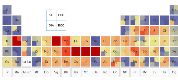
FIG. 5. Error decomposition for the original UZH settings. Left: SIRIUS-GTH-UZH relative to SIRIUS-FP-LAPW, which isolates the pseudopotential error. Right: CP2K-GTH-UZH relative to SIRIUS-GTH-UZH, which isolates the Gaussian-basis error.
