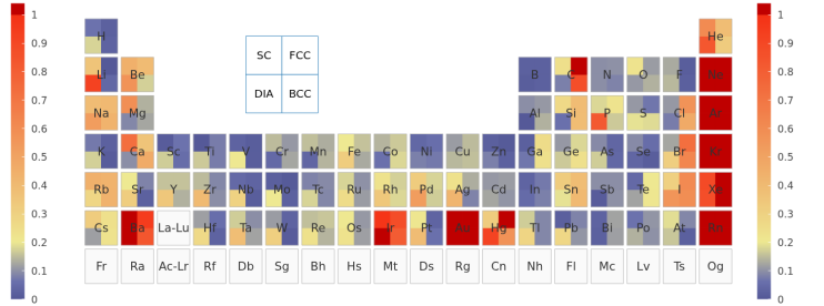
FIG. 5. Error decomposition for the original UZH settings. Left: SIRIUS-GTH-UZH relative to SIRIUS-FP-LAPW, which isolates the pseudopotential error. Right: CP2K-GTH-UZH relative to SIRIUS-GTH-UZH, which isolates the Gaussian-basis error.
