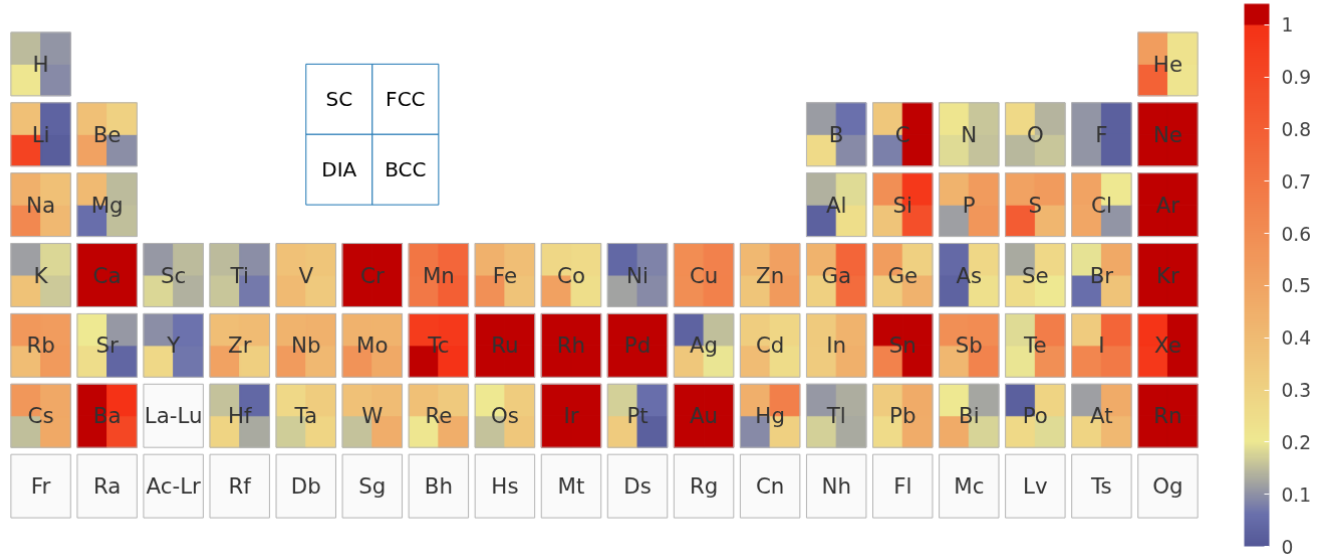
\epsilon for CP2K-GTH-UZH vs. SIRIUS-FP-LAPW
