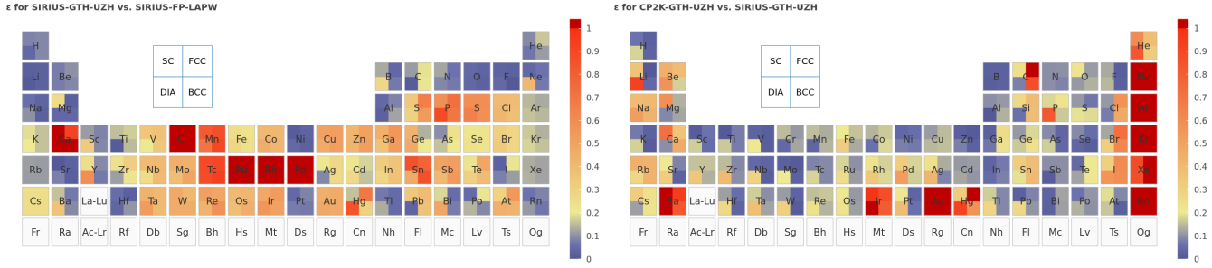
FIG. 5. Error decomposition for the original UZH settings. Right: CP2K-GTH-UZH relative to SIRIUS-GTH-UZH, which isolates the Gaussian-basis error. Left: SIRIUS-GTH-UZH relative to SIRIUS-FP-LAPW, which isolates the pseudopotential error.
