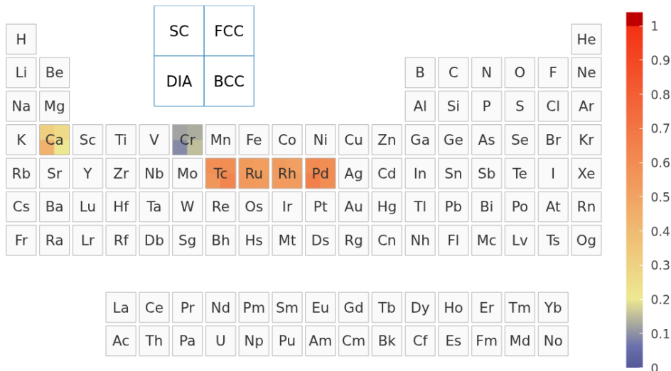
FIG. 6. Residual pseudopotential error for the improved UZH settings, obtained from SIRIUS-GTH-UZH-new relative to the SIRIUS-FP-LAPW reference.
