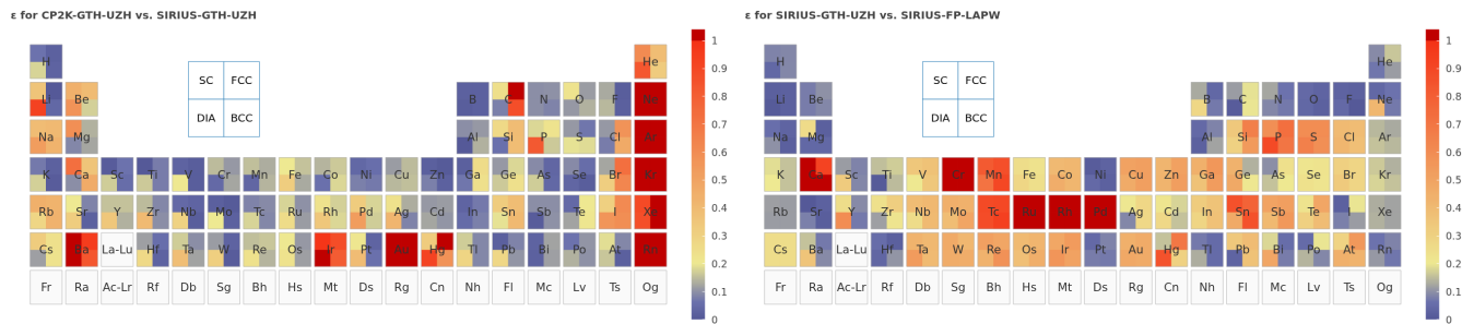
FIG. 5. Error decomposition for the original UZH settings. Left: CP2K-GTH-UZH relative to SIRIUS-GTH-UZH, which isolates the Gaussian-basis error. Right: SIRIUS-GTH-UZH relative to SIRIUS-FP-LAPW, which isolates the pseudopotential error.
