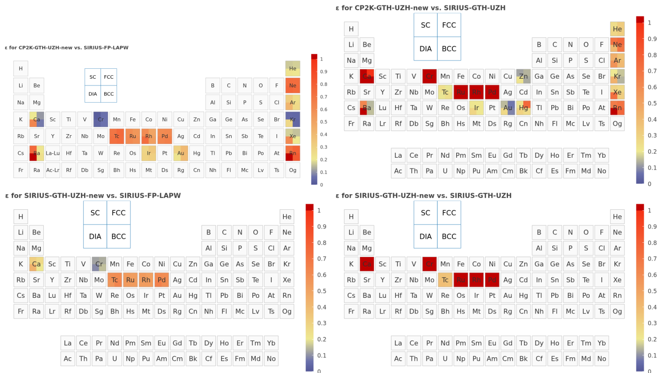
FIG. 6. Verification of the improved UZH settings. Top left: total CP2K-GTH-UZH-new error relative to SIRIUS-FP-LAPW. Top right: residual CP2K Gaussian-basis error. Bottom left: residual pseudopotential error after improvement. Bottom right: direct comparison of new and original SIRIUS-GTH-UZH pseudopotential settings.
