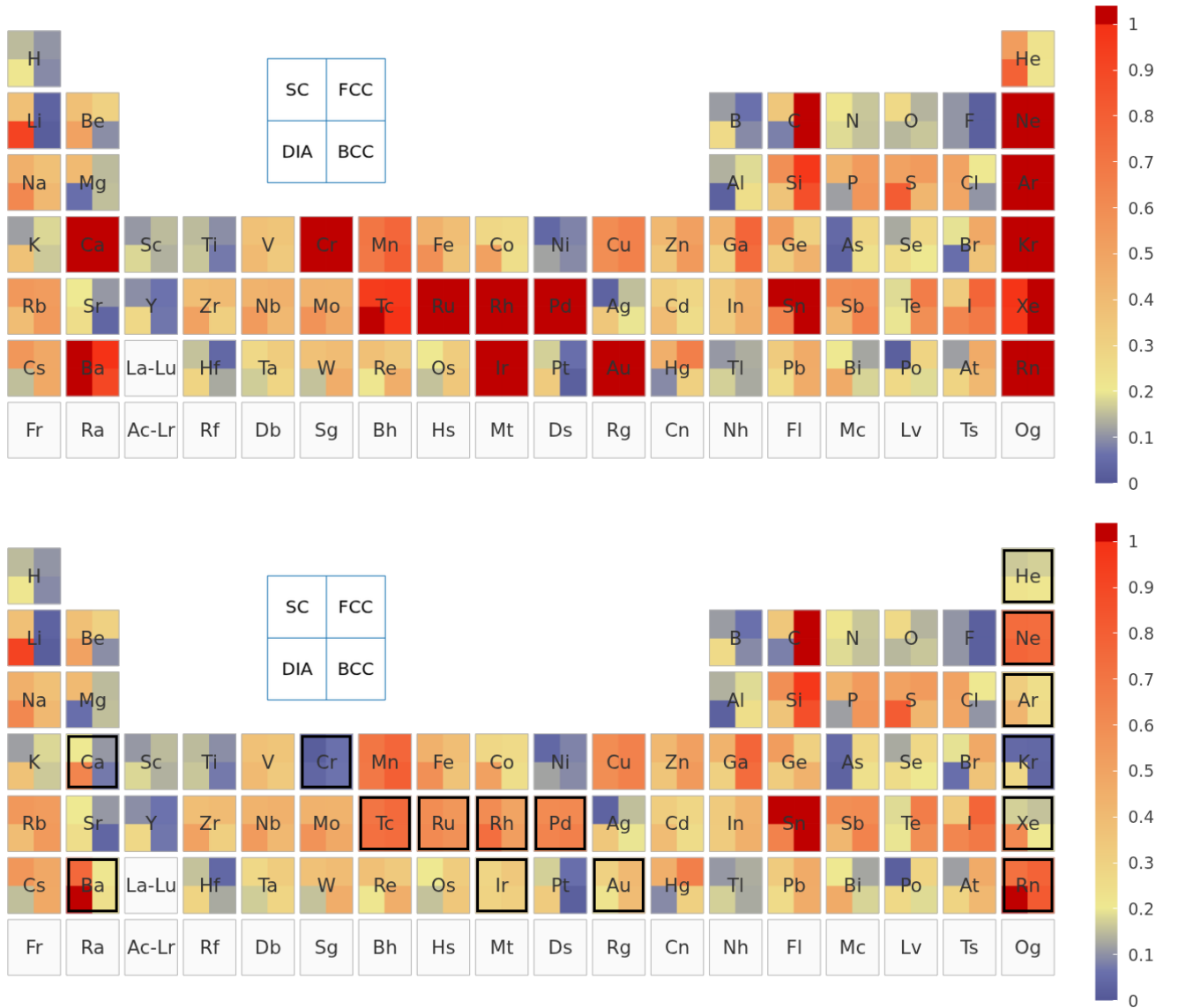
FIG. 4. Total equation-of-state error relative to SIRIUS-FP-LAPW, expressed with the \varepsilon metric of Eq. (10). Top: original CP2K-GTH-UZH settings. Bottom: completed view in which entries absent from the improved data set are filled with the corresponding original CP2K-GTH-UZH values; black frames mark the recomputed improved entries. Each map contains both Gaussian-basis and pseudopotential errors and therefore represents the practical production-level CP2K error before and after applying the UZH protocol.
