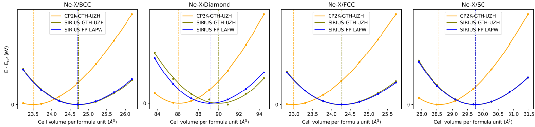
FIG. 5. Representative equation-of-state curves for Ne. Noble gases are sensitive tests of diffuse basis flexibility because their equation-of-state curves are shallow.
