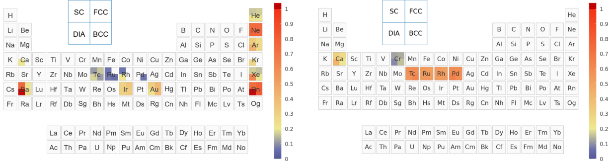
FIG. 6. Residual diagnostic for the improved settings. Left: residual CP2K Gaussian-basis contribution, constructed as the positive difference between the final CP2K-GTH-UZH-new total-error map and the residual pseudopotential map. Right: residual pseudopotential error for the improved SIRIUS-GTH-UZH-new settings relative to the SIRIUS-FP-LAPW reference. The left panel is a diagnostic estimate rather than a direct CP2K-GTH-UZH-new/SIRIUS-GTH-UZH-new equation-of-state comparison.
