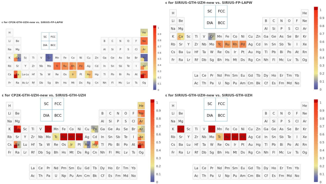
FIG. 6. Verification of the improved UZH settings. Top left : total CP2K-GTH-UZH-new error relative to SIRIUS-FP-LAPW. Bottom left : residual CP2K Gaussian-basis error. Top right : residual pseudopotential error after improvement. Bottom right : direct comparison of new and original SIRIUS-GTH-UZH pseudopotential settings.
