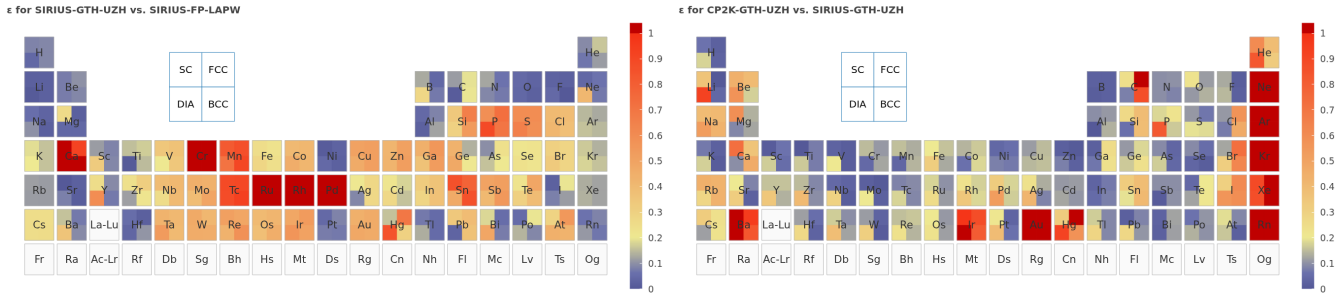
FIG. 5. Error decomposition for the original UZH settings. Left : SIRIUS-GTH-UZH relative to SIRIUS-FP-LAPW, which isolates the pseudopotential error. Right : CP2K-GTH-UZH relative to SIRIUS-GTH-UZH, which isolates the Gaussian-basis error.
