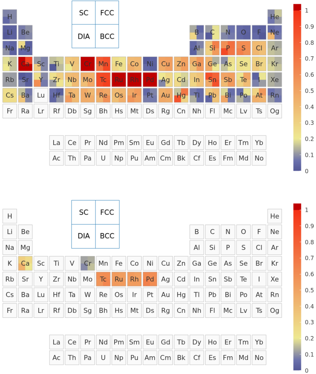
FIG. 7. Pseudopotential contribution before and after applying the UZH protocol. Top: original SIRSUS-GTH-UZH settings relative to SIRSUS-FP-LAPW. Bottom: improved SIRSUS-GTH-UZH-new settings relative to SIRSUS-FP-LAPW. Because both panels use SIRSUS on the pseudopotential side, the CP2K Gaussian basis is absent and the comparison isolates the pseudopotential transferability error.
