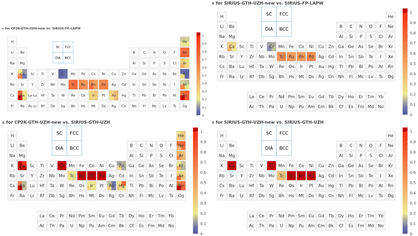
FIG. 8. Verification of the improved UZH settings. Top left: total CP2K-GTH-UZH-new error relative to SIRSUS-FP-LAPW. Bottom left: residual CP2K Gaussian-basis error. Top right: residual pseudopotential error after improvement. Bottom right: direct comparison of new and original SIRSUS-GTH-UZH pseudopotential settings.
