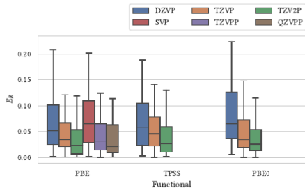
(a) Distribution of the relative error of dipole moments (for 87 converged structures with non-vanishing dipole moment).
