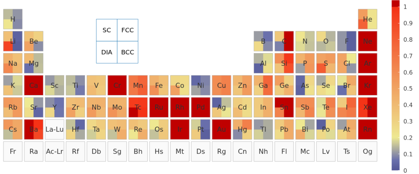
FIG. 4. Total equation-of-state error of the original CP2K-GTH-UZH settings relative to SIRIUS-FP-LAPW, expressed with the \varepsilon metric of Eq. (11). This comparison contains both Gaussian-basis and pseudopotential errors.
