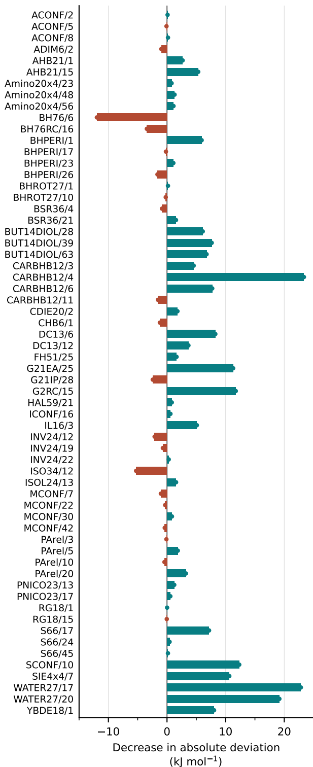
(a) Benchmark reference 42/62 smaller deviations
