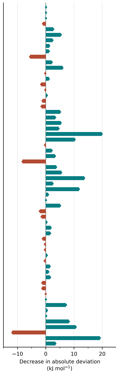
(b) GauXC-AE 43/62 smaller deviations
