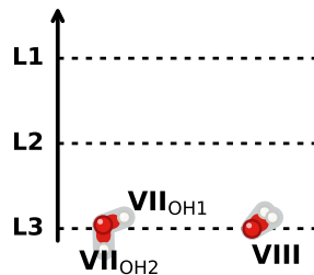
L3 / motif VIII second-layer H-bonded water
