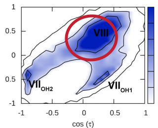
total SFG fingerprint VIII
