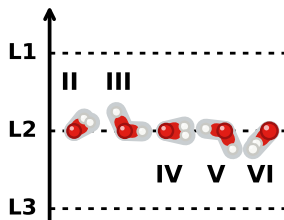
L2 / motif VI H-bonded bridge
