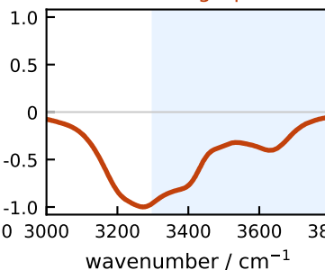
total SFG fingerprint VI
