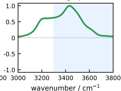
total SFG fingerprint VIII
