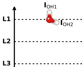
a L1 / motif I weak/free OH toward SiO 2
