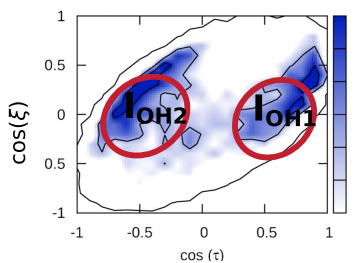
c total SFG fingerprint I
