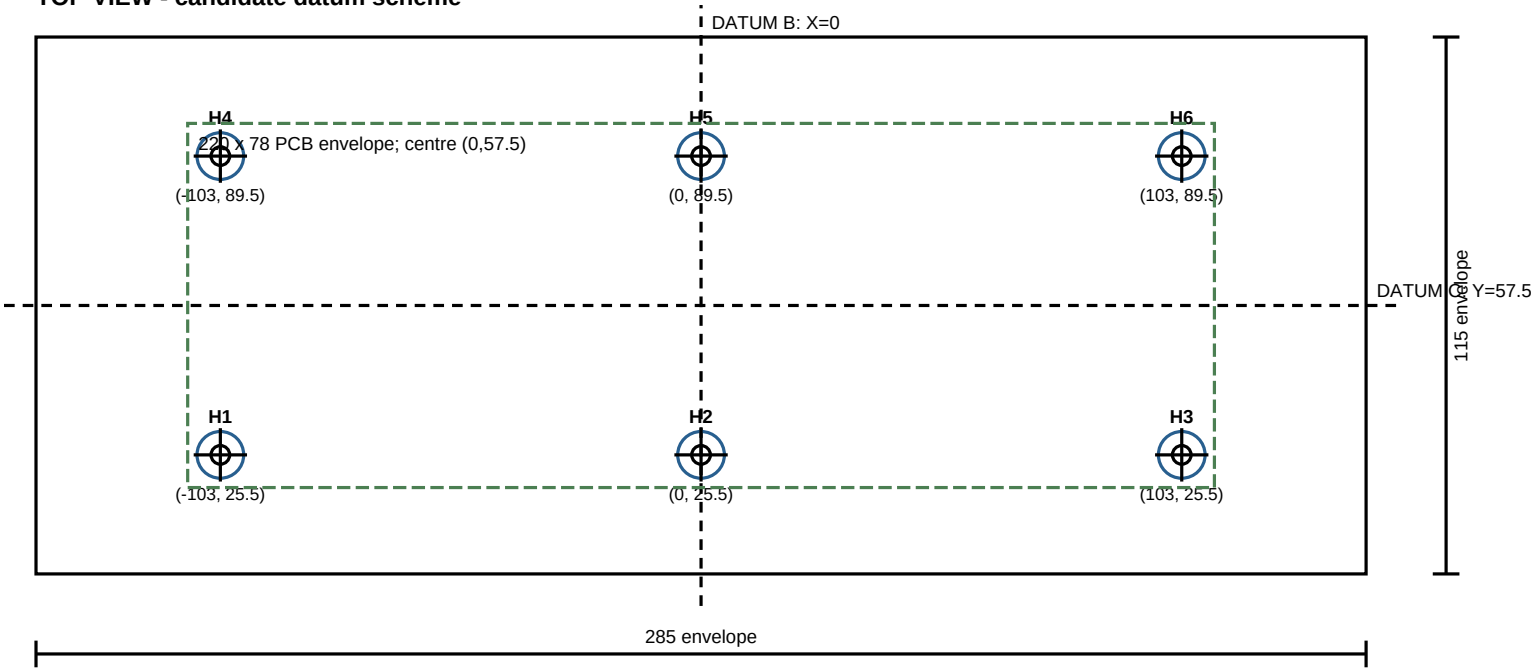
TOP VIEW - candidate datum scheme
