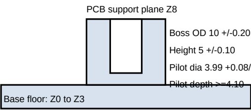
SECTION A-A - candidate boss
