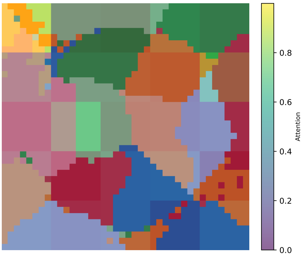
Attention + Antennas
