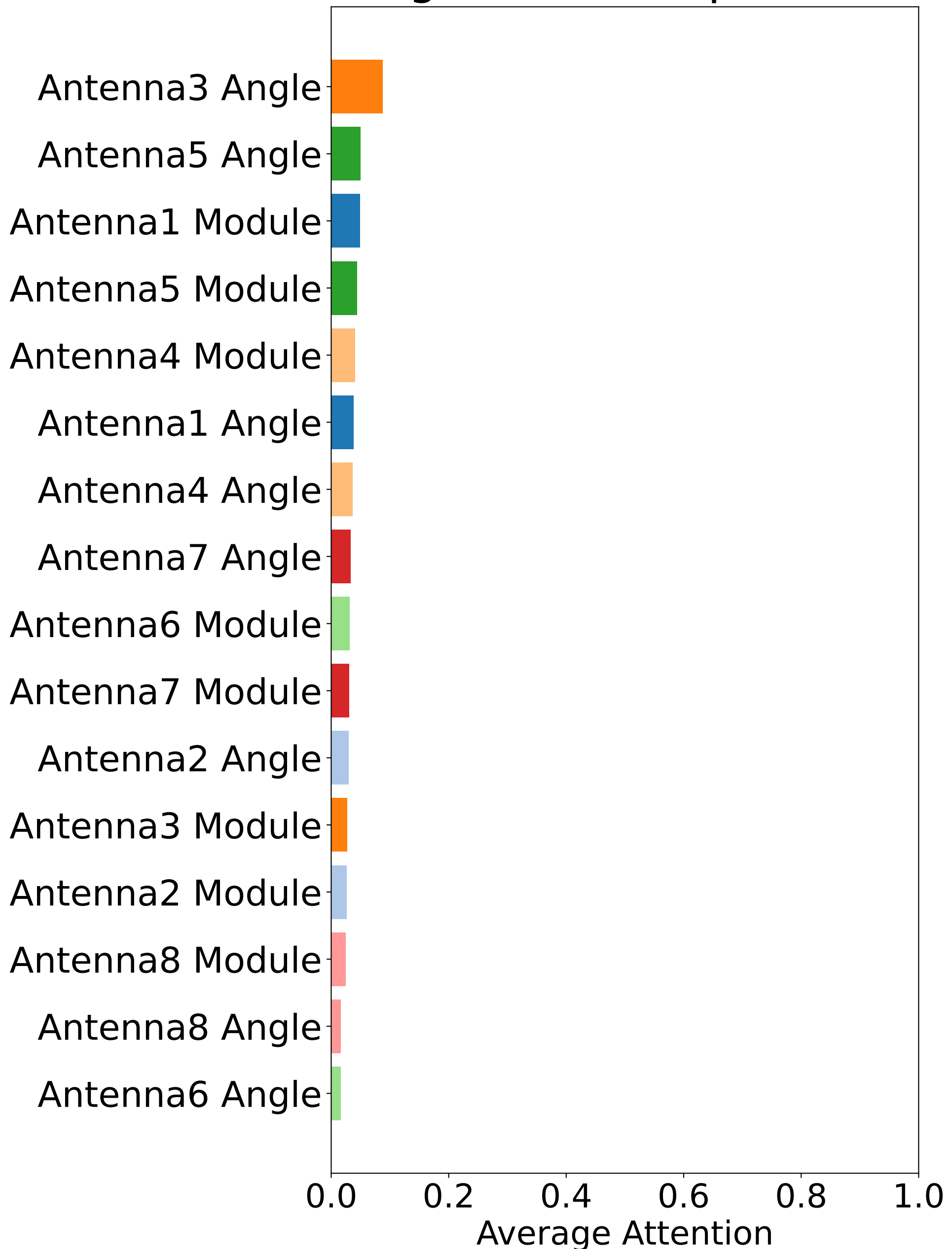
Average Attention per Feature
