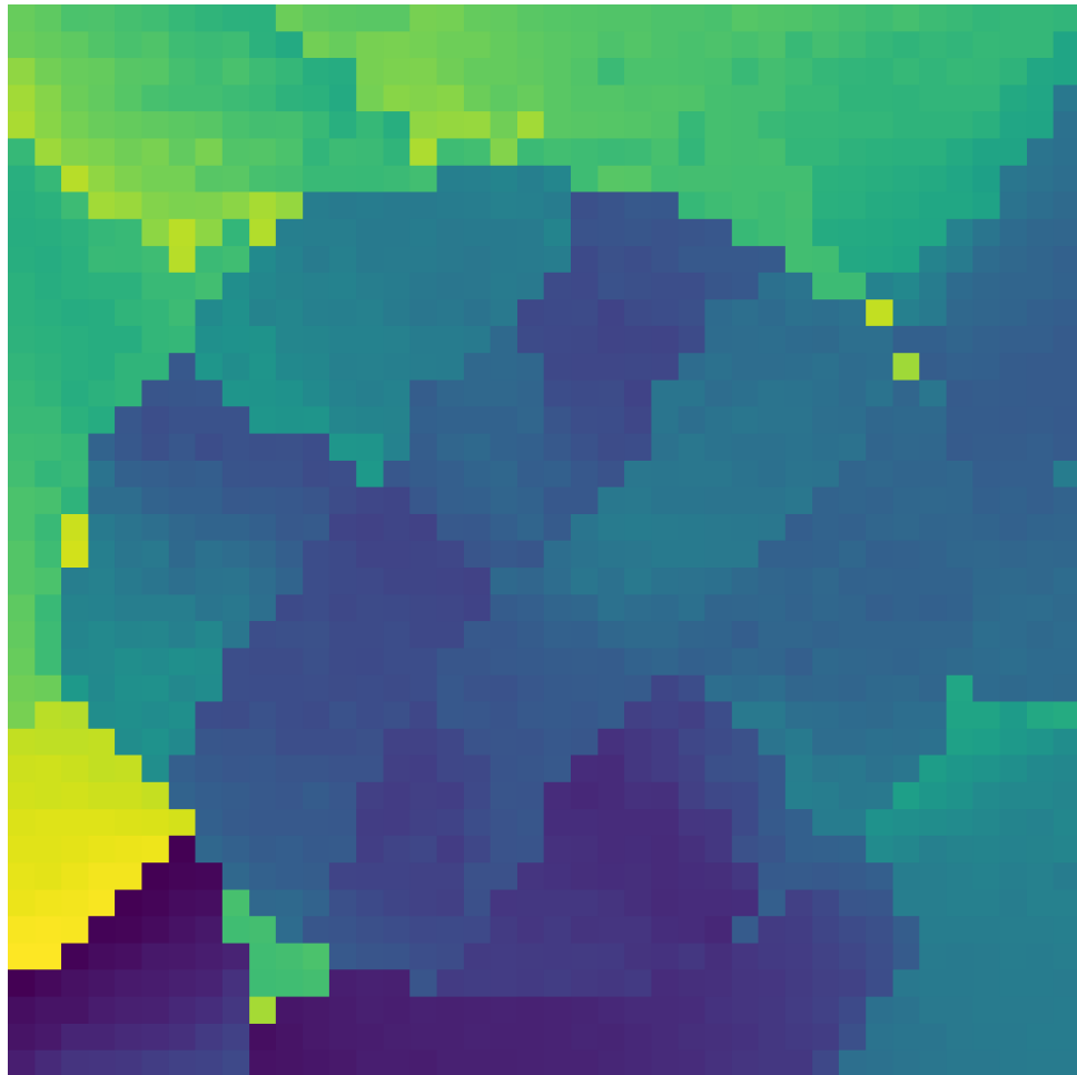
Original Image
