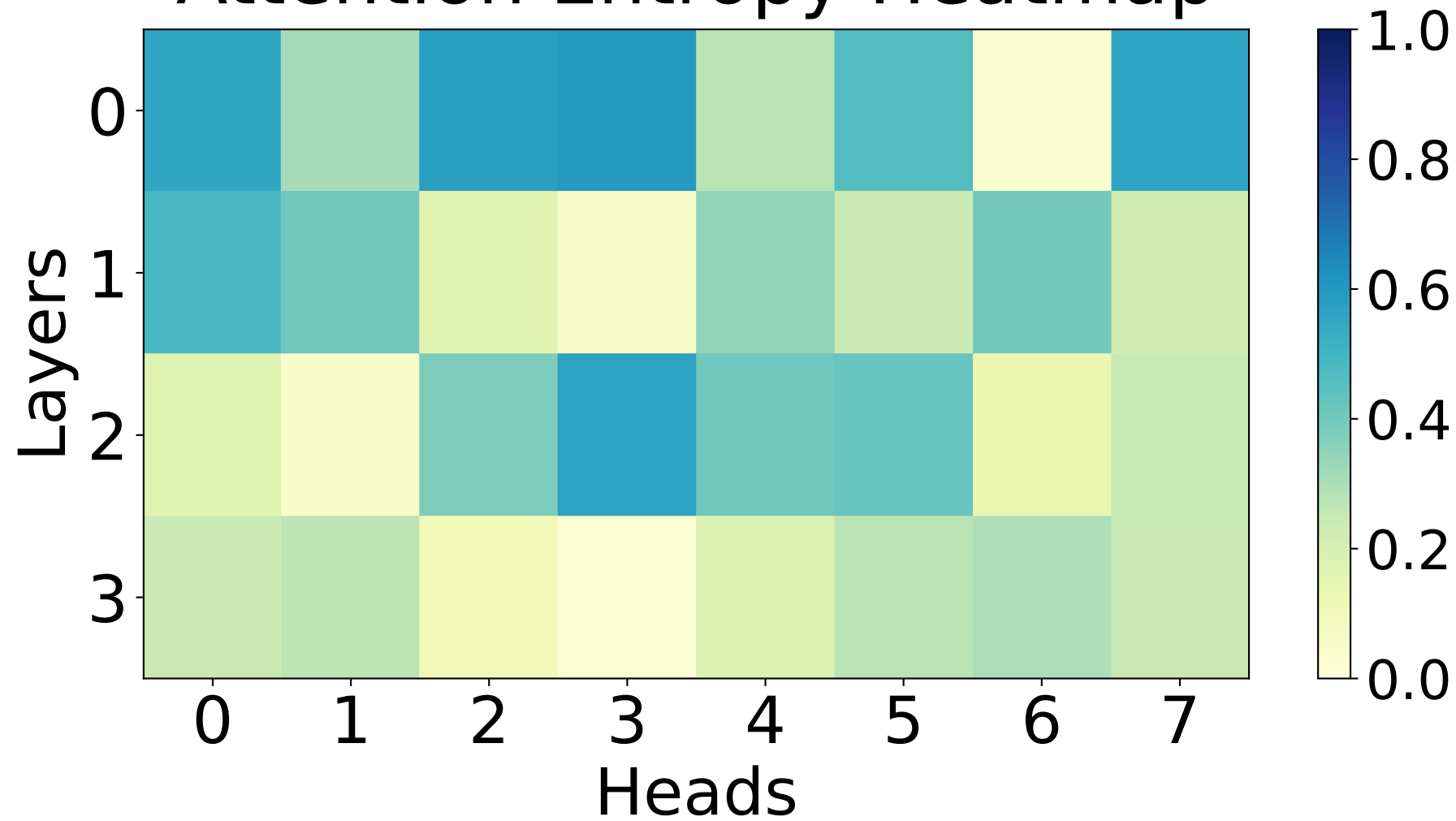
Attention Entropy Heatmap
