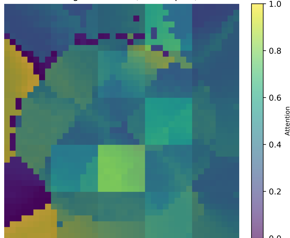
Average Attention (All Samples)
