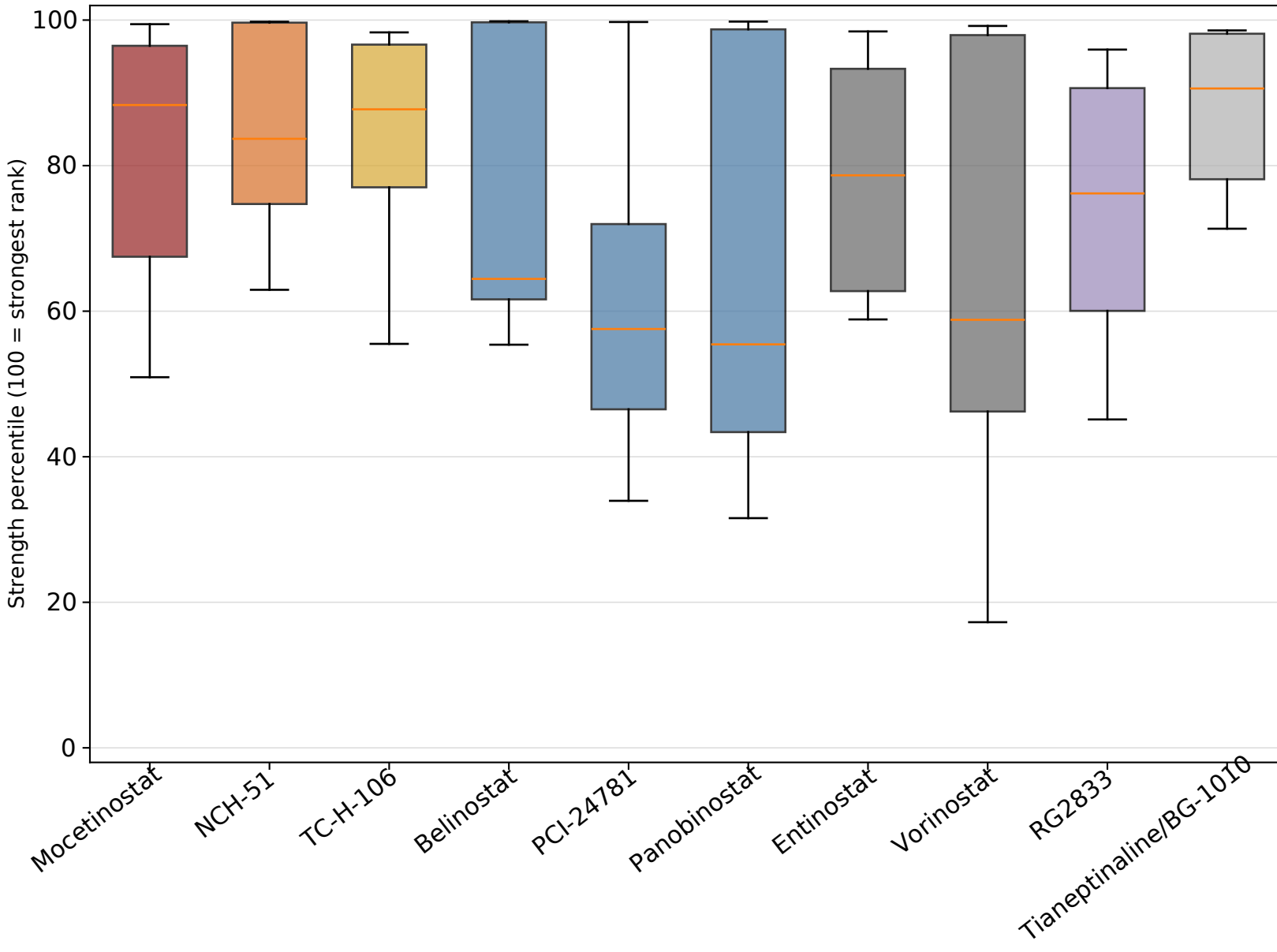
A Primary 48-config stability: signed wTRS + Spearman reversal
