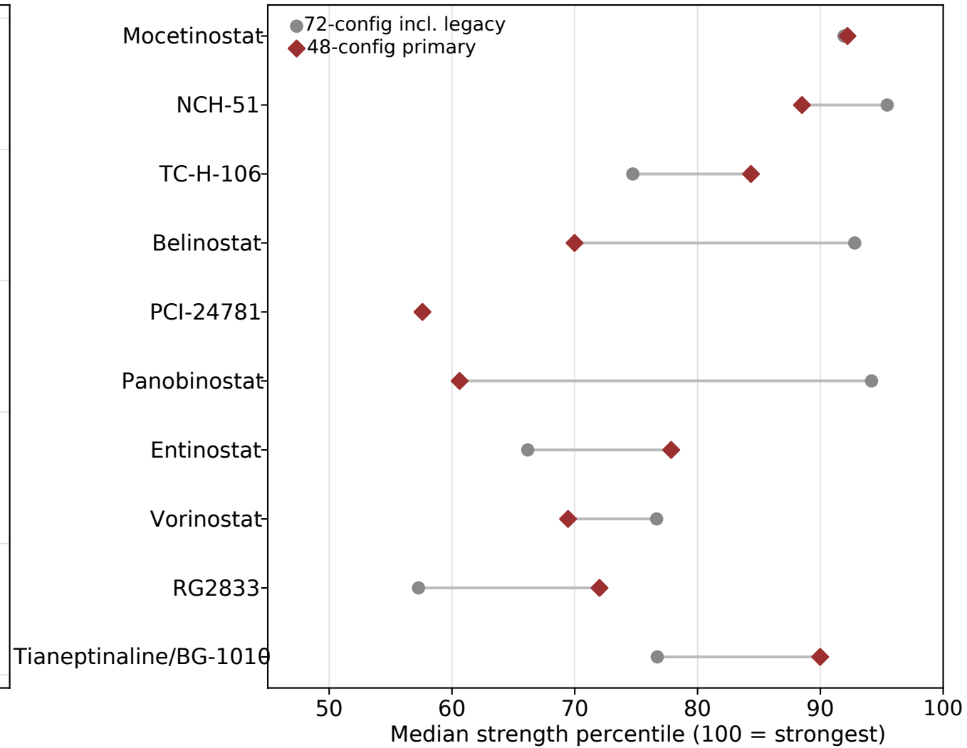
B Primary versus legacy-inclusive summary
